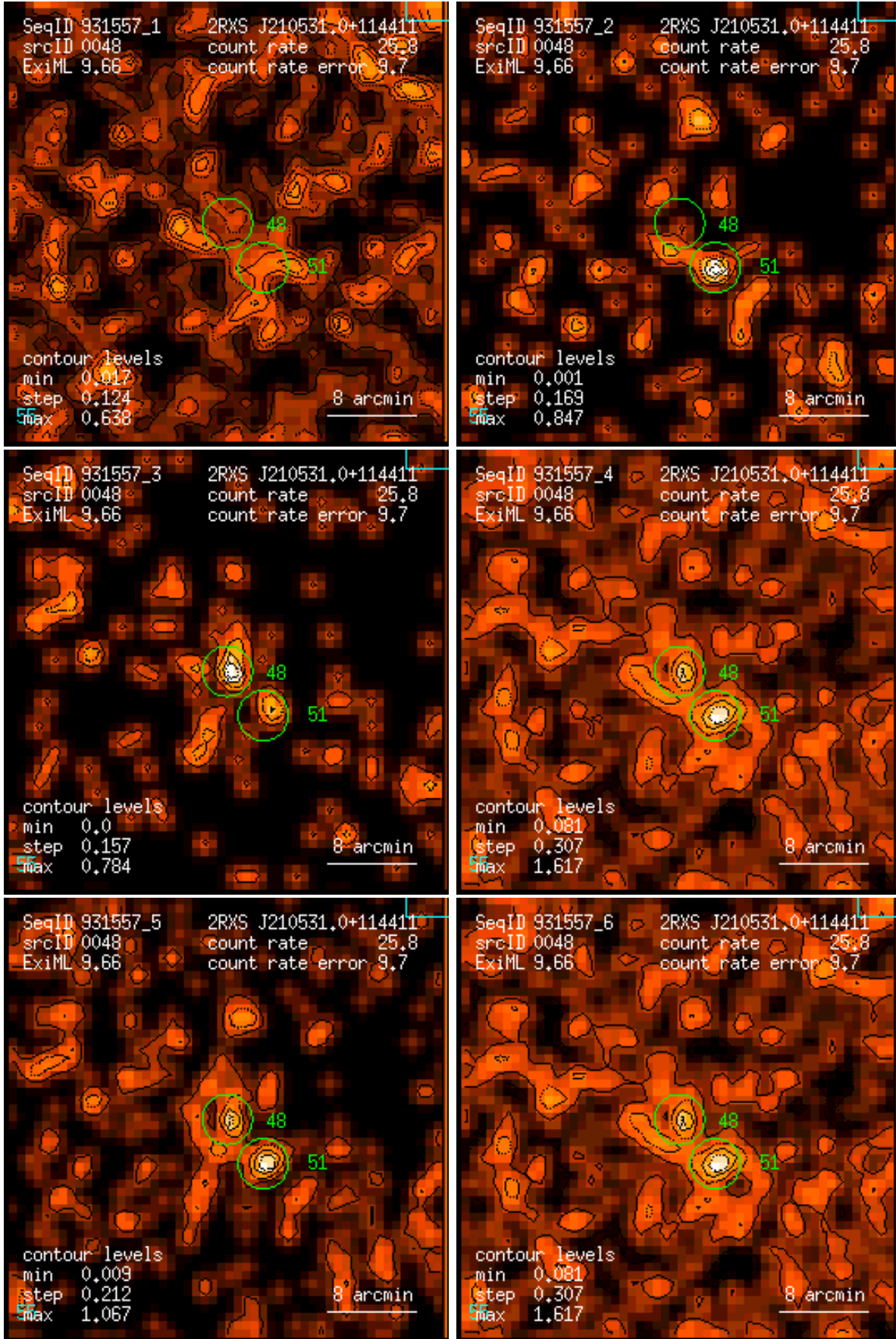
Figure 48: RASS 931557: detection 0048: band rate images, Gaussian filter: (1) PSPC channels 11 – 41, (2) 52 – 90, (3) 91 – 201, (4) 11 – 235, (5) 52 – 201, (6) 11 – 201. Broad band rates in counts/ks. Band rate contour levels in counts/ks/arcmin 2 .
