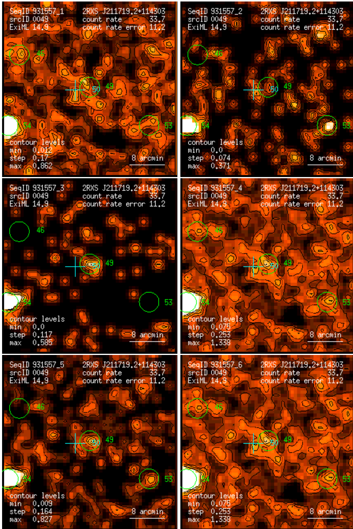
Figure 49: RASS 931557: detection 0049: band rate images, Gaussian filter: (1) PSPC channels 11 – 41, (2) 52 – 90, (3) 91 – 201, (4) 11 – 235, (5) 52 – 201, (6) 11 – 201. Broad band rates in counts/ks. Band rate contour levels in counts/ks/arcmin 2 .
