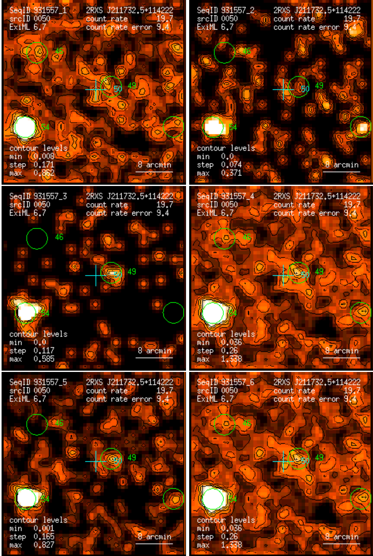
Figure 50: RASS 931557: detection 0050: band rate images, Gaussian filter: (1) PSPC channels 11 – 41, (2) 52 – 90, (3) 91 – 201, (4) 11 – 235, (5) 52 – 201, (6) 11 – 201. Broad band rates in counts/ks. Band rate contour levels in counts/ks/arcmin 2 .
