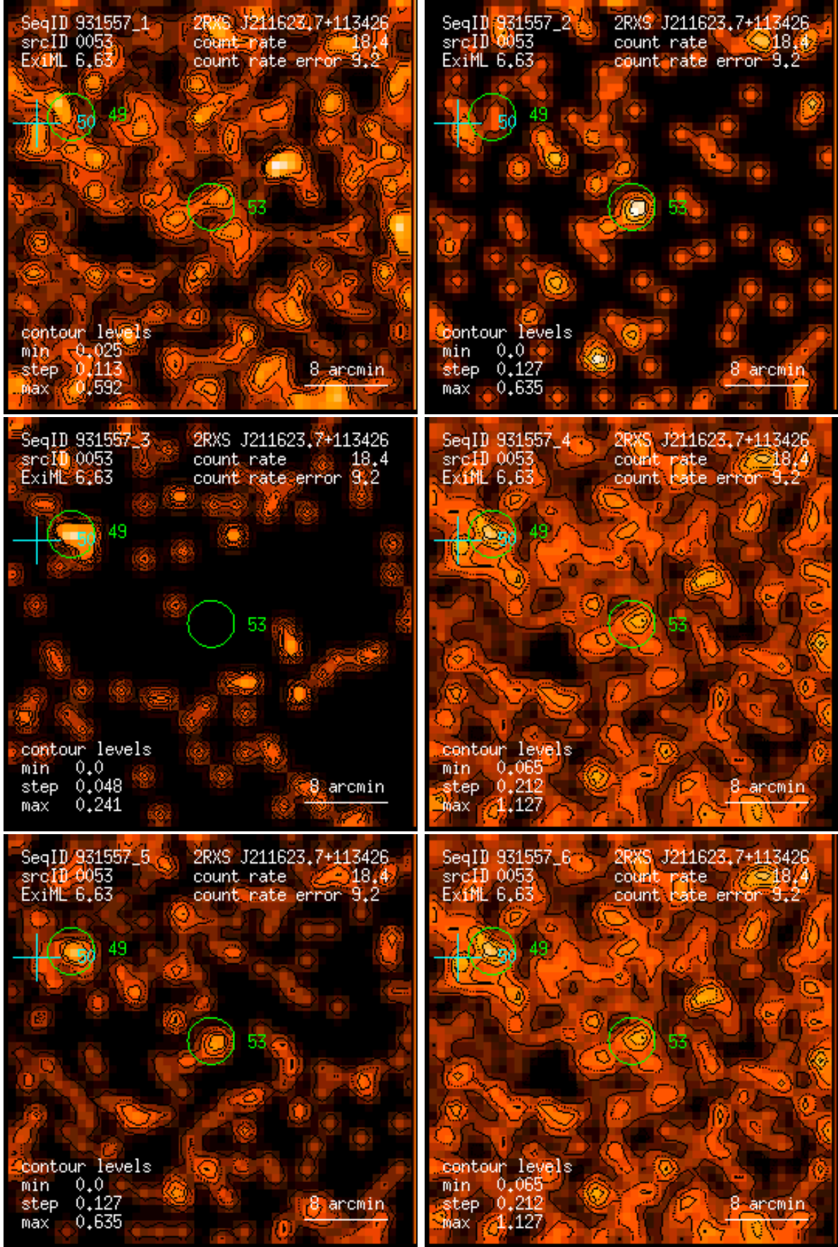
Figure 53: RASS 931557: detection 0053: band rate images, Gaussian filter: (1) PSPC channels 11 – 41, (2) 52 – 90, (3) 91 – 201, (4) 11 – 235, (5) 52 – 201, (6) 11 – 201. Broad band rates in counts/ks. Band rate contour levels in counts/ks/arcmin 2 .
