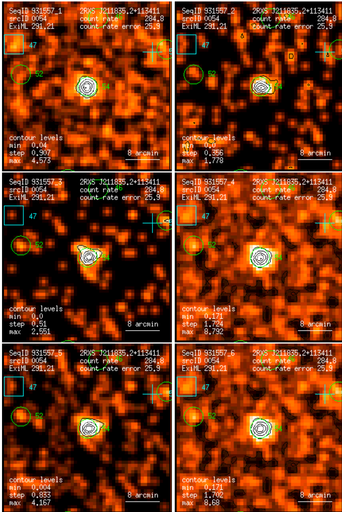
Figure 54: RASS 931557: detection 0054: band rate images, Gaussian filter: (1) PSPC channels 11 – 41, (2) 52 – 90, (3) 91 – 201, (4) 11 – 235, (5) 52 – 201, (6) 11 – 201. Broad band rates in counts/ks. Band rate contour levels in counts/ks/arcmin 2 .
