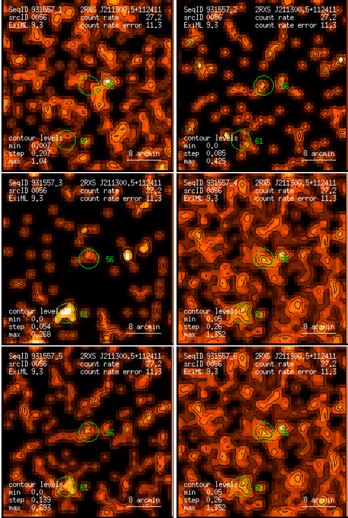
Figure 56: RASS 931557: detection 0056: band rate images, Gaussian filter: (1) PSPC channels 11 – 41, (2) 52 – 90, (3) 91 – 201, (4) 11 – 235, (5) 52 – 201, (6) 11 – 201. Broad band rates in counts/ks. Band rate contour levels in counts/ks/arcmin 2 .
