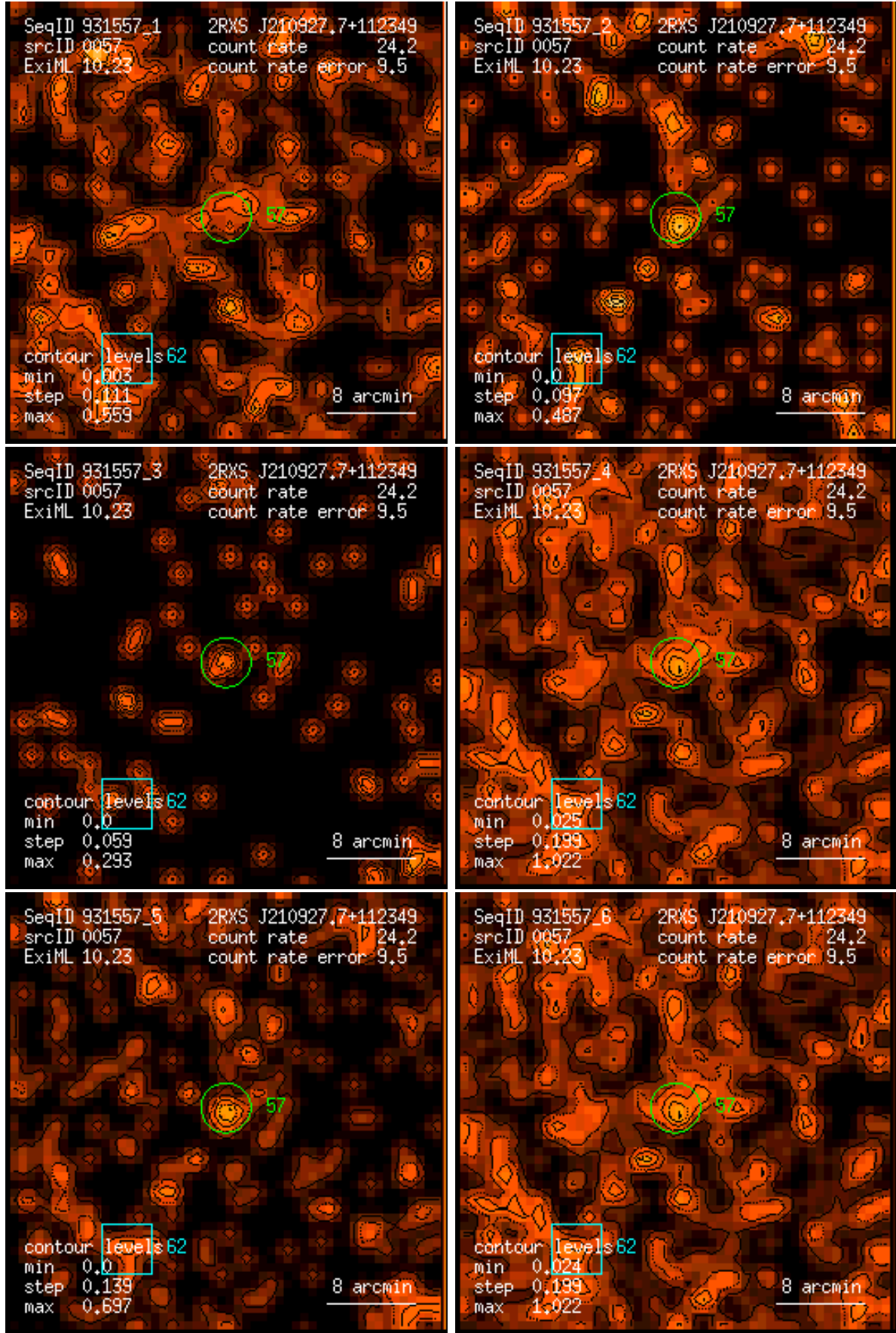
Figure 57: RASS 931557: detection 0057: band rate images, Gaussian filter: (1) PSPC channels 11 – 41, (2) 52 – 90, (3) 91 – 201, (4) 11 – 235, (5) 52 – 201, (6) 11 – 201. Broad band rates in counts/ks. Band rate contour levels in counts/ks/arcmin 2 .
