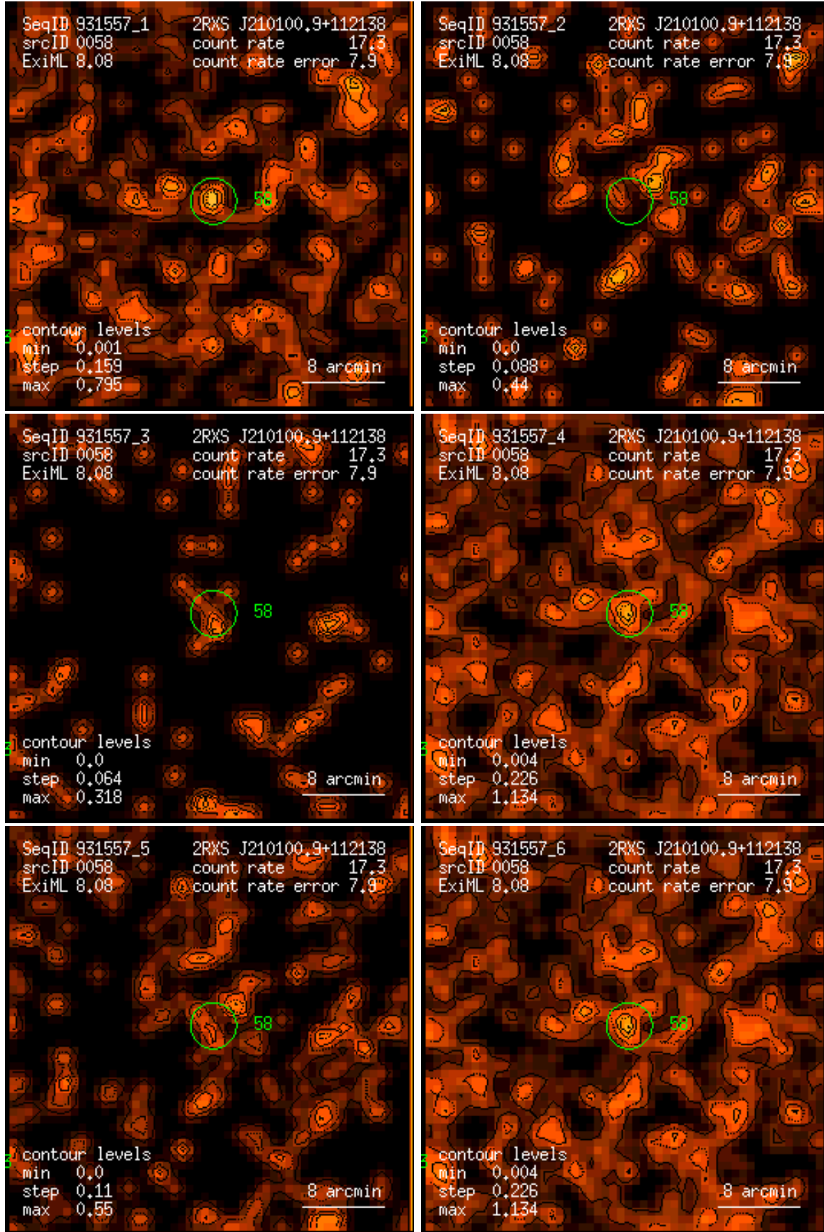
Figure 58: RASS 931557: detection 0058: band rate images, Gaussian filter: (1) PSPC channels 11 – 41, (2) 52 – 90, (3) 91 – 201, (4) 11 – 235, (5) 52 – 201, (6) 11 – 201. Broad band rates in counts/ks. Band rate contour levels in counts/ks/arcmin 2 .
