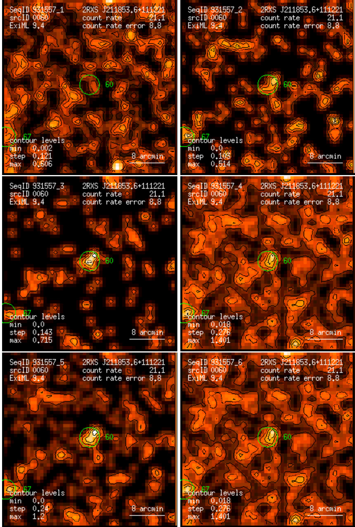
Figure 60: RASS 931557: detection 0060: band rate images, Gaussian filter: (1) PSPC channels 11 – 41, (2) 52 – 90, (3) 91 – 201, (4) 11 – 235, (5) 52 – 201, (6) 11 – 201. Broad band rates in counts/ks. Band rate contour levels in counts/ks/arcmin 2 .
