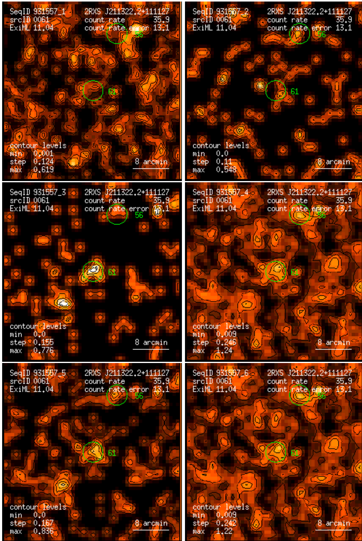
Figure 61: RASS 931557: detection 0061: band rate images, Gaussian filter: (1) PSPC channels 11 – 41, (2) 52 – 90, (3) 91 – 201, (4) 11 – 235, (5) 52 – 201, (6) 11 – 201. Broad band rates in counts/ks. Band rate contour levels in counts/ks/arcmin 2 .
