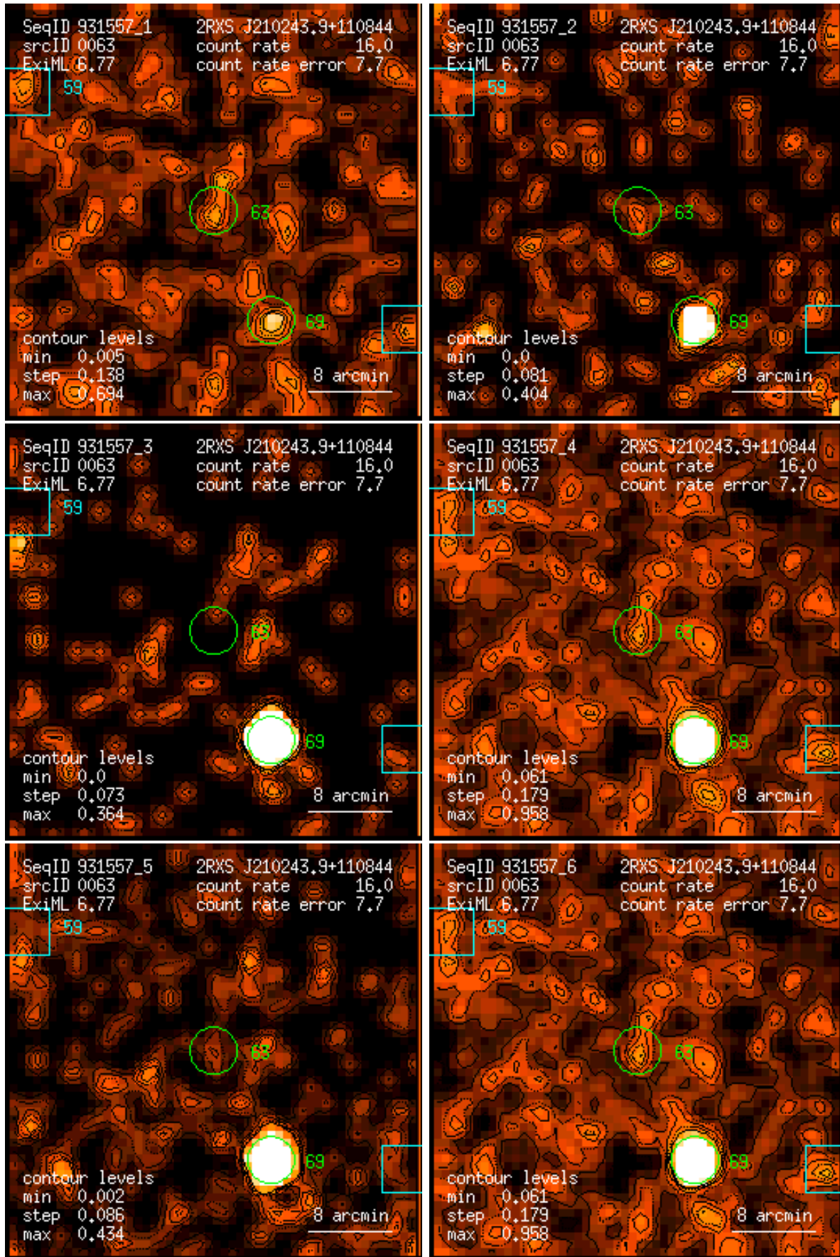
Figure 63: RASS 931557: detection 0063: band rate images, Gaussian filter: (1) PSPC channels 11 – 41, (2) 52 – 90, (3) 91 – 201, (4) 11 – 235, (5) 52 – 201, (6) 11 – 201. Broad band rates in counts/ks. Band rate contour levels in counts/ks/arcmin 2 .
