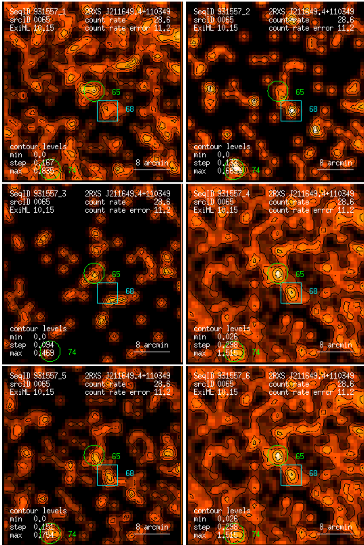
Figure 65: RASS 931557: detection 0065: band rate images, Gaussian filter: (1) PSPC channels 11 – 41, (2) 52 – 90, (3) 91 – 201, (4) 11 – 235, (5) 52 – 201, (6) 11 – 201. Broad band rates in counts/ks. Band rate contour levels in counts/ks/arcmin 2 .
