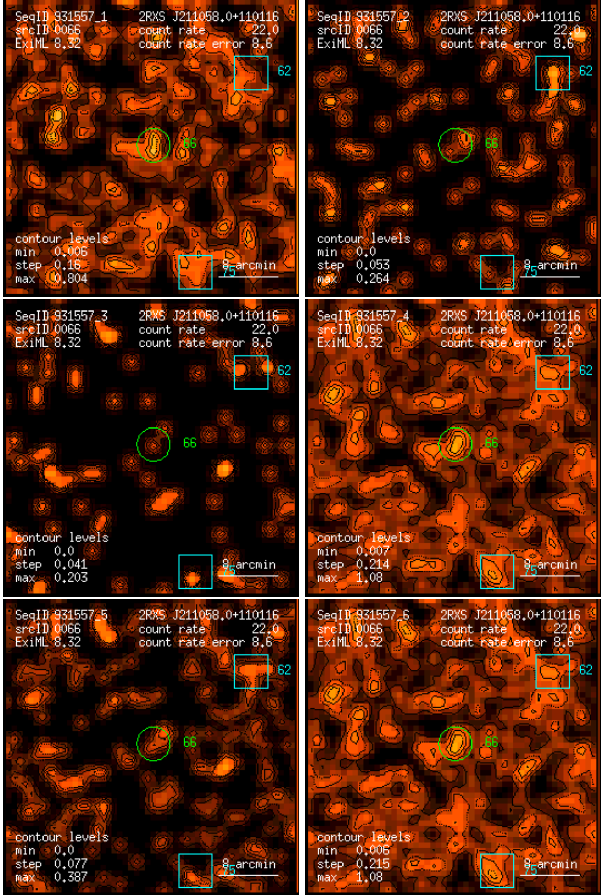
Figure 66: RASS 931557: detection 0066: band rate images, Gaussian filter: (1) PSPC channels 11 – 41, (2) 52 – 90, (3) 91 – 201, (4) 11 – 235, (5) 52 – 201, (6) 11 – 201. Broad band rates in counts/ks. Band rate contour levels in counts/ks/arcmin 2 .
