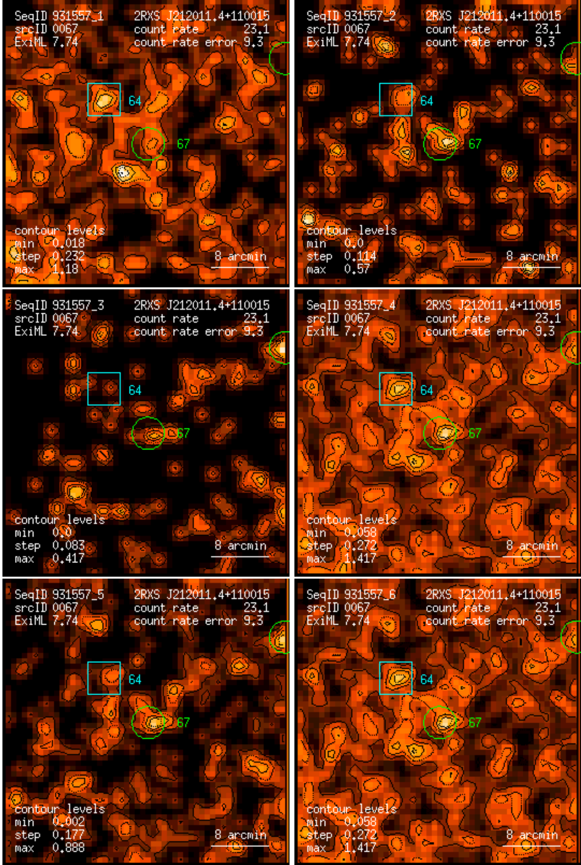
Figure 67: RASS 931557: detection 0067: band rate images, Gaussian filter: (1) PSPC channels 11 – 41, (2) 52 – 90, (3) 91 – 201, (4) 11 – 235, (5) 52 – 201, (6) 11 – 201. Broad band rates in counts/ks. Band rate contour levels in counts/ks/arcmin 2 .
