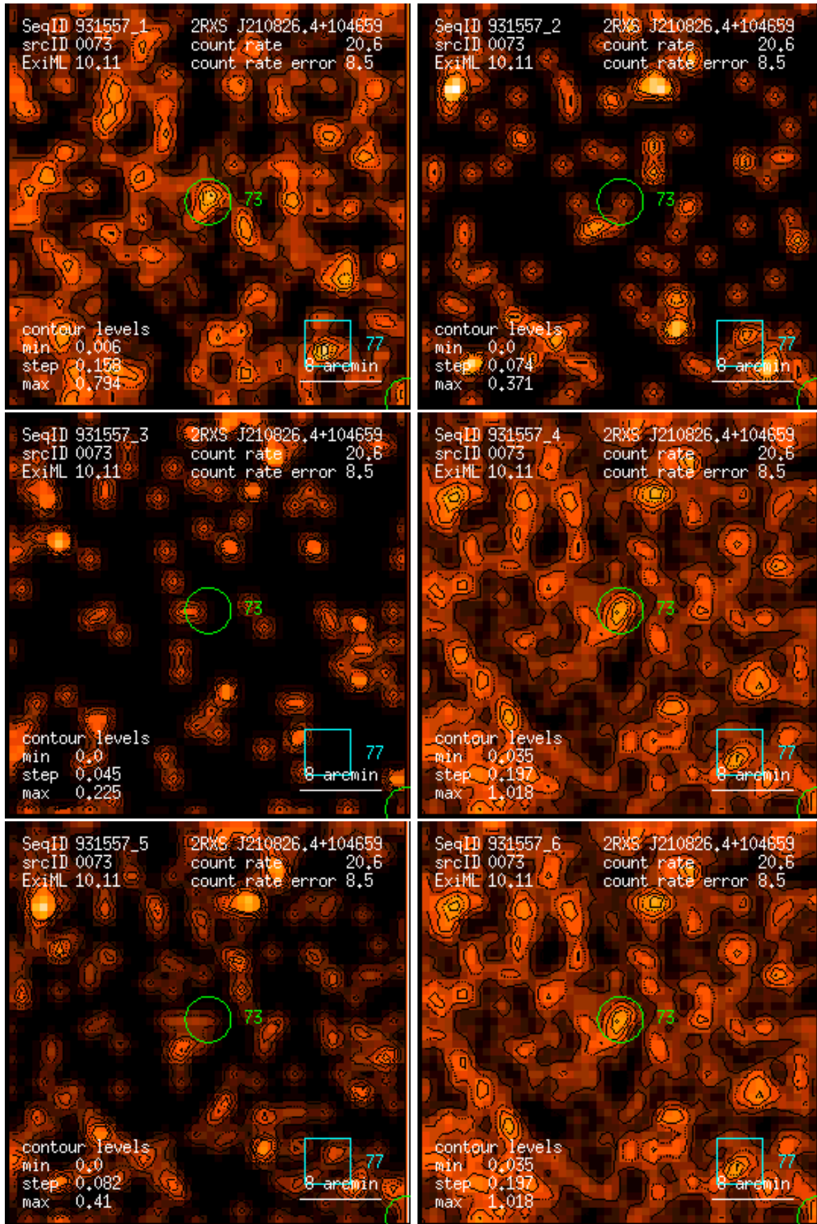
Figure 73: RASS 931557: detection 0073: band rate images, Gaussian filter: (1) PSPC channels 11 – 41, (2) 52 – 90, (3) 91 – 201, (4) 11 – 235, (5) 52 – 201, (6) 11 – 201. Broad band rates in counts/ks. Band rate contour levels in counts/ks/arcmin 2 .
