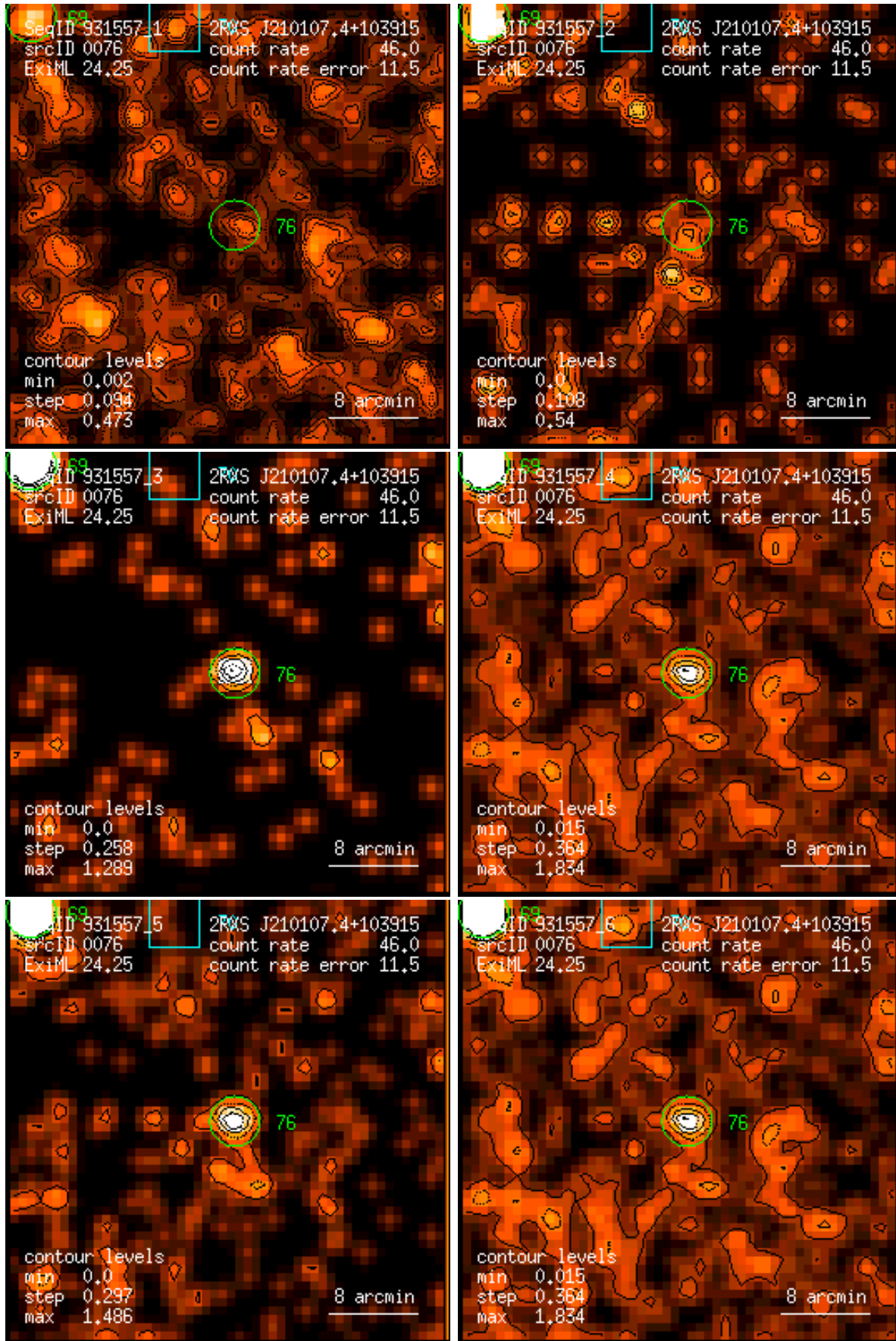
Figure 76: RASS 931557: detection 0076: band rate images, Gaussian filter: (1) PSPC channels 11 – 41, (2) 52 – 90, (3) 91 – 201, (4) 11 – 235, (5) 52 – 201, (6) 11 – 201. Broad band rates in counts/ks. Band rate contour levels in counts/ks/arcmin 2 .
