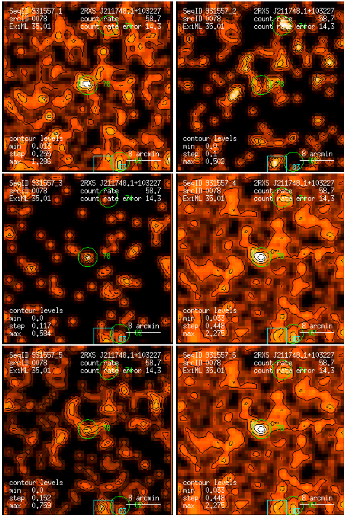
Figure 78: RASS 931557: detection 0078: band rate images, Gaussian filter: (1) PSPC channels 11 – 41, (2) 52 – 90, (3) 91 – 201, (4) 11 – 235, (5) 52 – 201, (6) 11 – 201. Broad band rates in counts/ks. Band rate contour levels in counts/ks/arcmin 2 .
