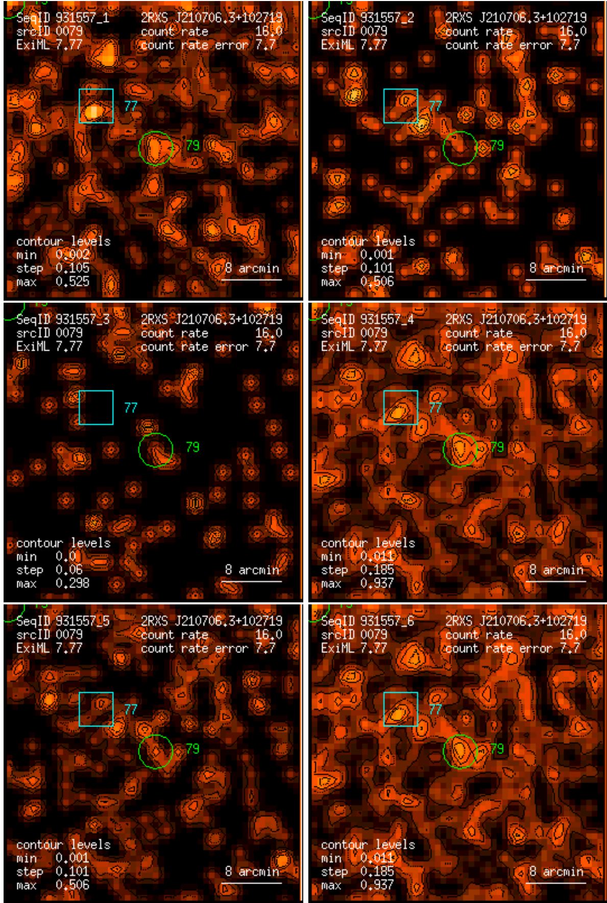
Figure 79: RASS 931557: detection 0079: band rate images, Gaussian filter: (1) PSPC channels 11 – 41, (2) 52 – 90, (3) 91 – 201, (4) 11 – 235, (5) 52 – 201, (6) 11 – 201. Broad band rates in counts/ks. Band rate contour levels in counts/ks/arcmin 2 .
