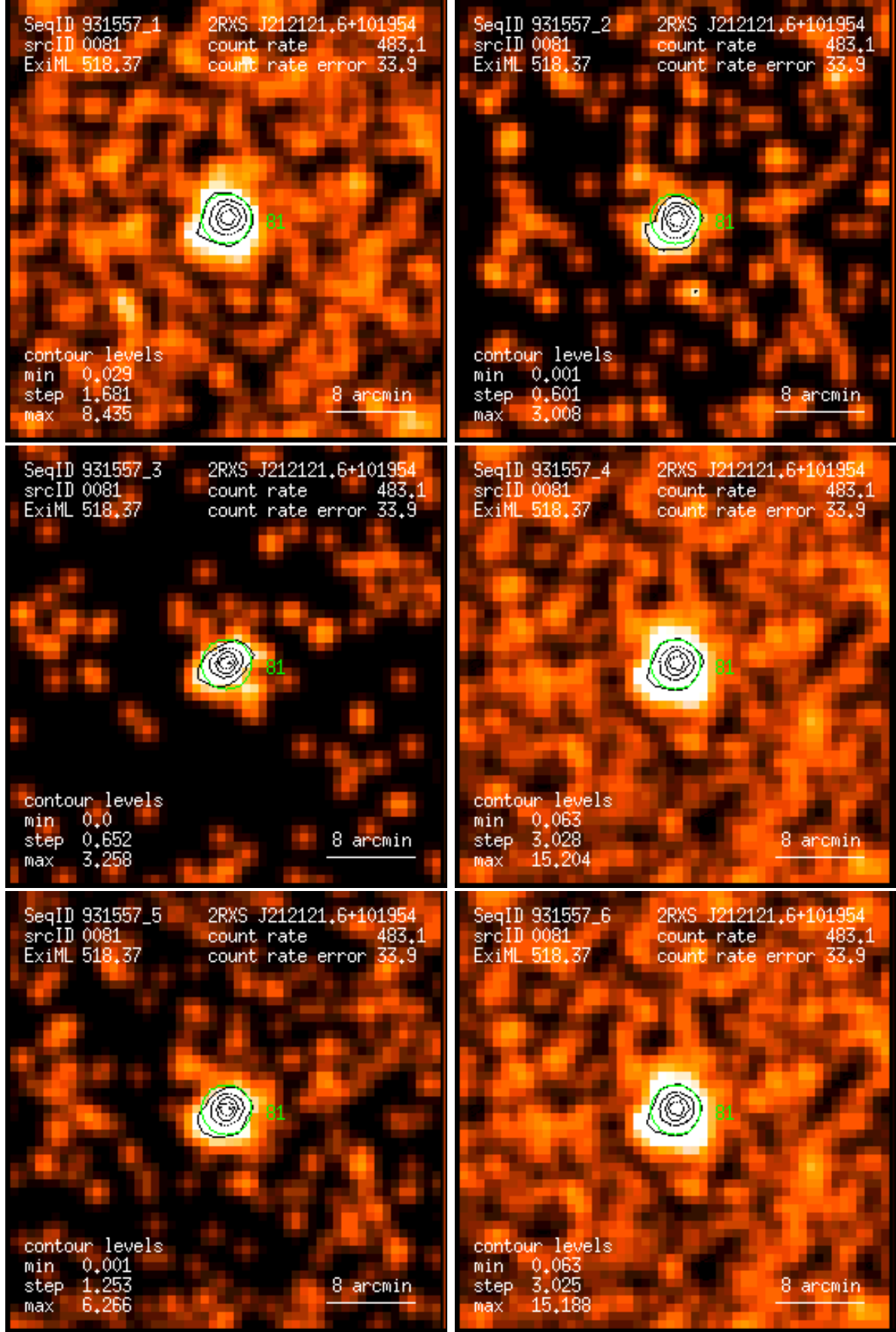
Figure 81: RASS 931557: detection 0081: band rate images, Gaussian filter: (1) PSPC channels 11 – 41, (2) 52 – 90, (3) 91 – 201, (4) 11 – 235, (5) 52 – 201, (6) 11 – 201. Broad band rates in counts/ks. Band rate contour levels in counts/ks/arcmin 2 .
