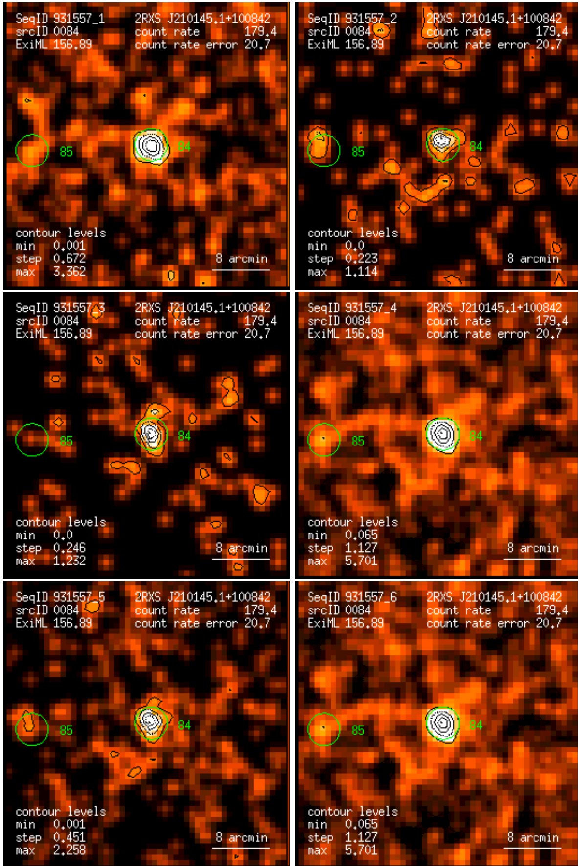
Figure 84: RASS 931557: detection 0084: band rate images, Gaussian filter: (1) PSPC channels 11 – 41, (2) 52 – 90, (3) 91 – 201, (4) 11 – 235, (5) 52 – 201, (6) 11 – 201. Broad band rates in counts/ks. Band rate contour levels in counts/ks/arcmin 2 .
