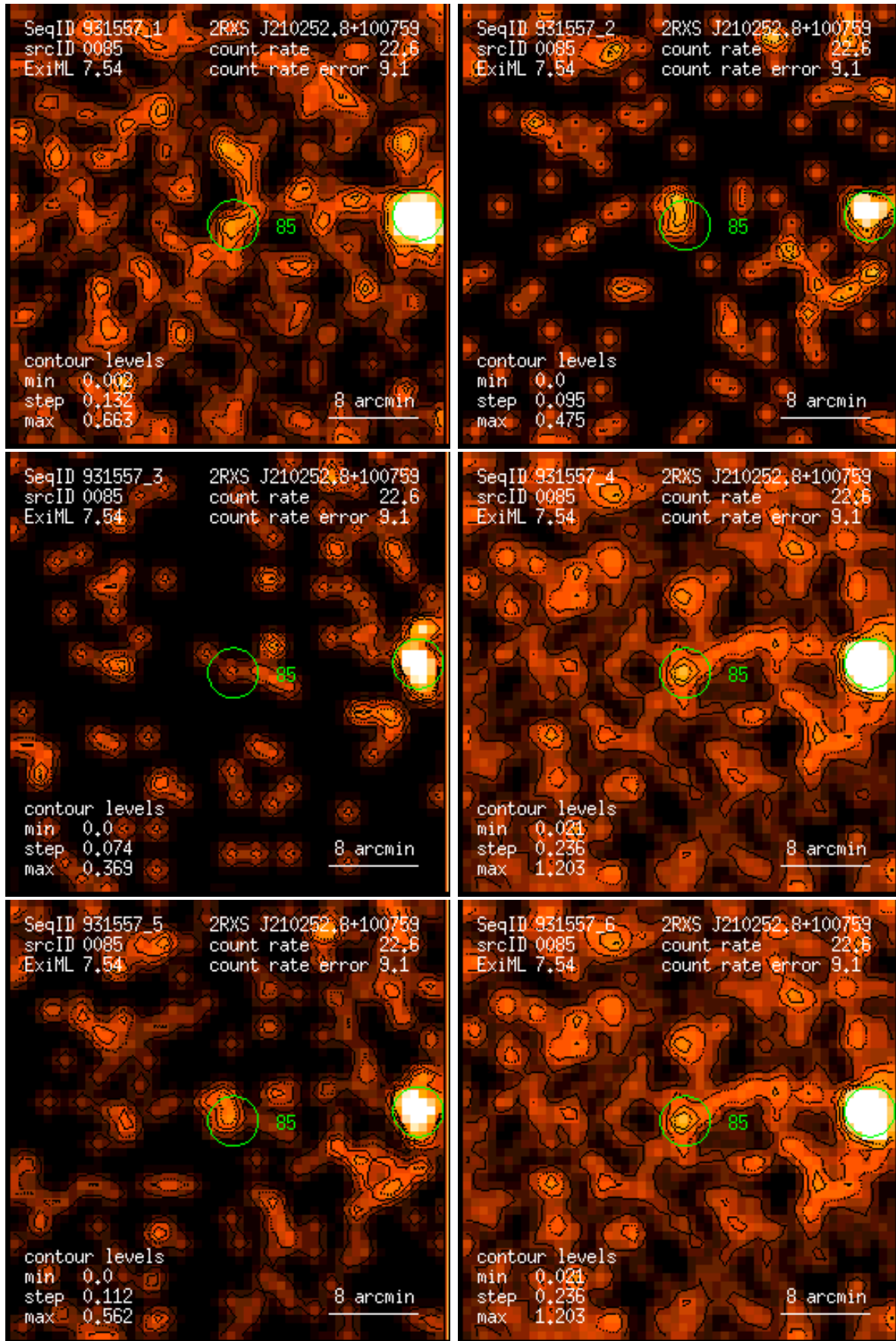
Figure 85: RASS 931557: detection 0085: band rate images, Gaussian filter: (1) PSPC channels 11 – 41, (2) 52 – 90, (3) 91 – 201, (4) 11 – 235, (5) 52 – 201, (6) 11 – 201. Broad band rates in counts/ks. Band rate contour levels in counts/ks/arcmin 2 .
