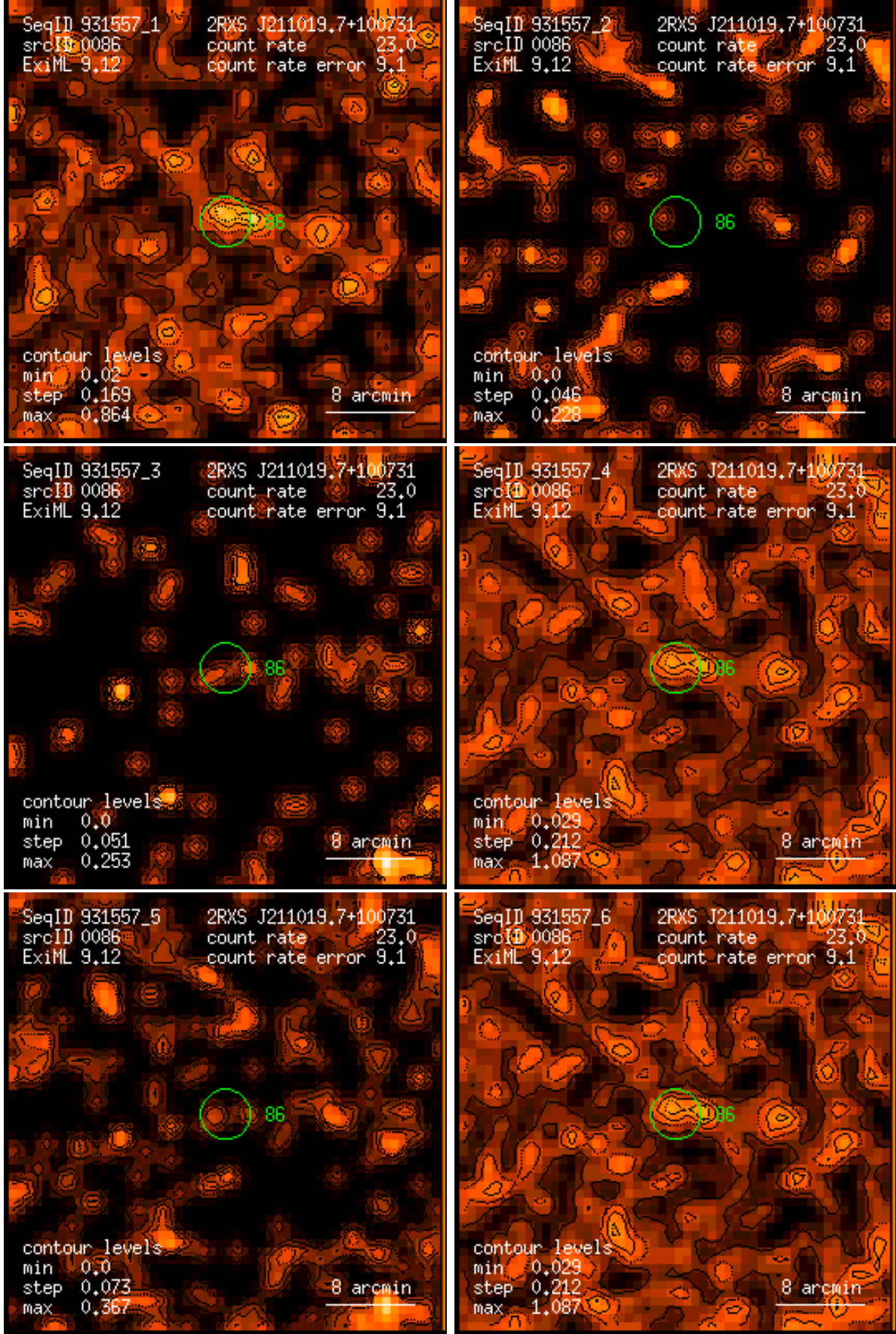
Figure 86: RASS 931557: detection 0086: band rate images, Gaussian filter: (1) PSPC channels 11 – 41, (2) 52 – 90, (3) 91 – 201, (4) 11 – 235, (5) 52 – 201, (6) 11 – 201. Broad band rates in counts/ks. Band rate contour levels in counts/ks/arcmin 2 .
