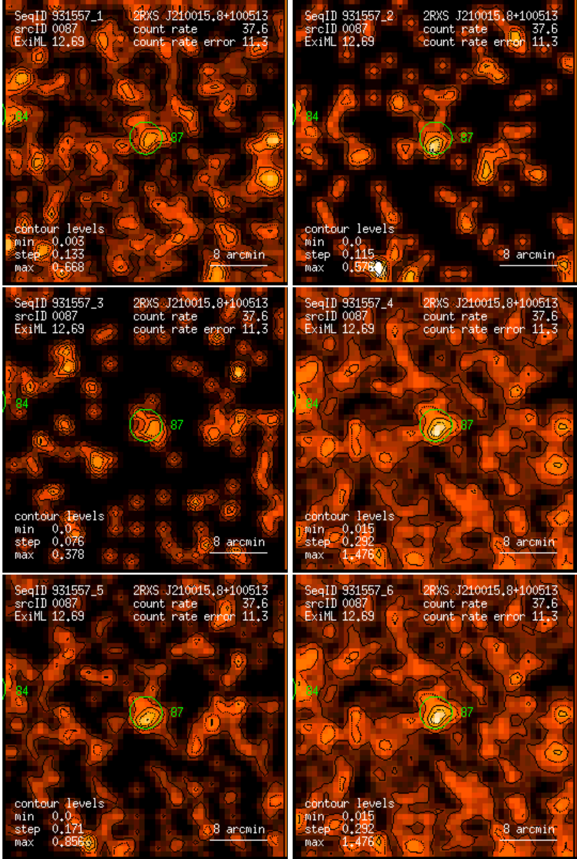
Figure 87: RASS 931557: detection 0087: band rate images, Gaussian filter: (1) PSPC channels 11 – 41, (2) 52 – 90, (3) 91 – 201, (4) 11 – 235, (5) 52 – 201, (6) 11 – 201. Broad band rates in counts/ks. Band rate contour levels in counts/ks/arcmin 2 .
