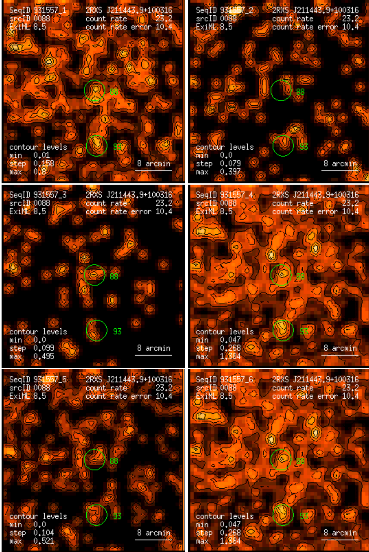
Figure 88: RASS 931557: detection 0088: band rate images, Gaussian filter: (1) PSPC channels 11 – 41, (2) 52 – 90, (3) 91 – 201, (4) 11 – 235, (5) 52 – 201, (6) 11 – 201. Broad band rates in counts/ks. Band rate contour levels in counts/ks/arcmin 2 .
