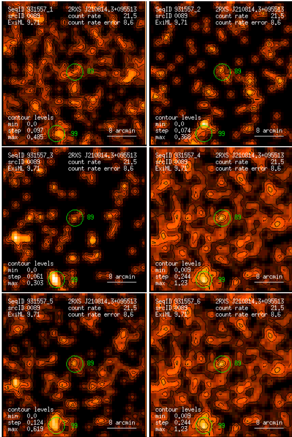
Figure 89: RASS 931557: detection 0089: band rate images, Gaussian filter: (1) PSPC channels 11 – 41, (2) 52 – 90, (3) 91 – 201, (4) 11 – 235, (5) 52 – 201, (6) 11 – 201. Broad band rates in counts/ks. Band rate contour levels in counts/ks/arcmin 2 .
