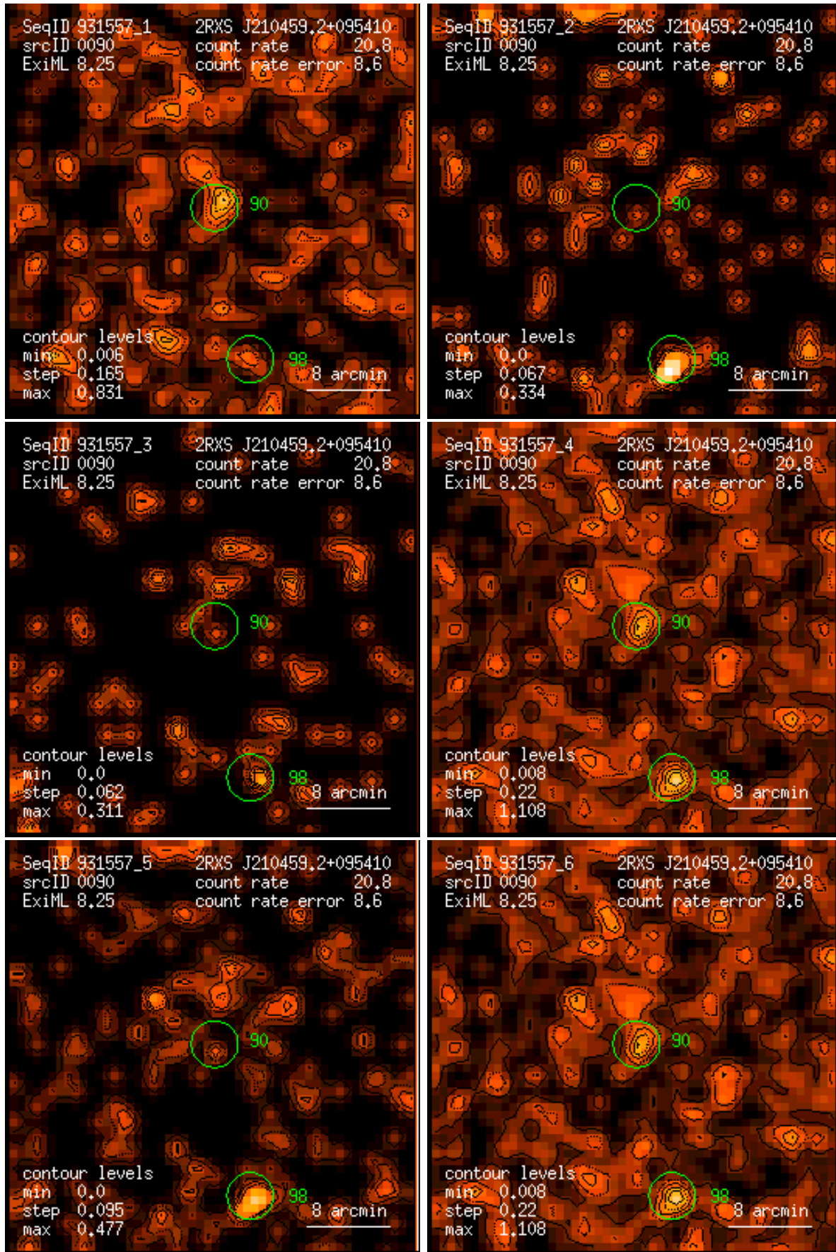
Figure 90: RASS 931557: detection 0090: band rate images, Gaussian filter: (1) PSPC channels 11 – 41, (2) 52 – 90, (3) 91 – 201, (4) 11 – 235, (5) 52 – 201, (6) 11 – 201. Broad band rates in counts/ks. Band rate contour levels in counts/ks/arcmin 2 .
