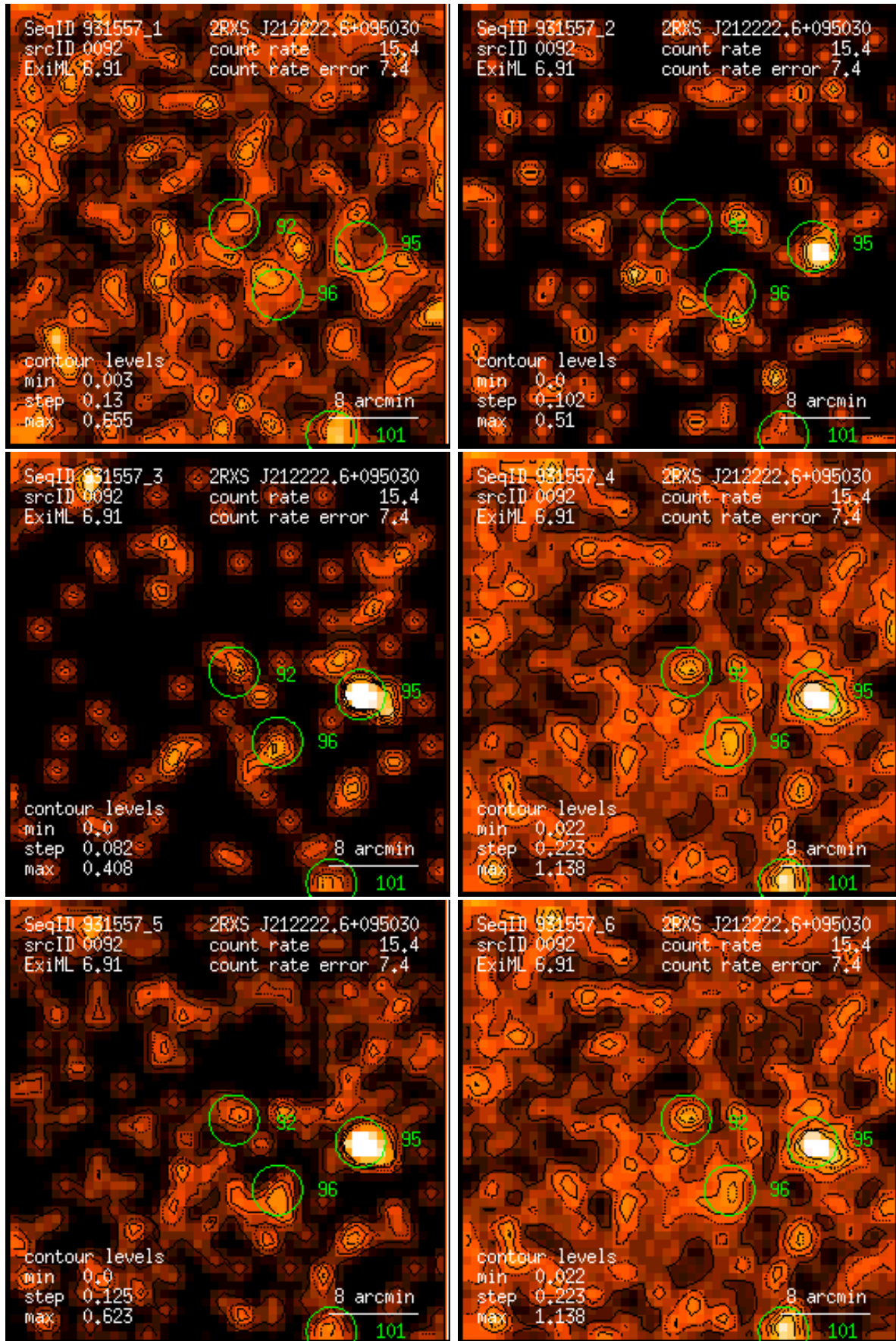
Figure 92: RASS 931557: detection 0092: band rate images, Gaussian filter: (1) PSPC channels 11 – 41, (2) 52 – 90, (3) 91 – 201, (4) 11 – 235, (5) 52 – 201, (6) 11 – 201. Broad band rates in counts/ks. Band rate contour levels in counts/ks/arcmin 2 .
