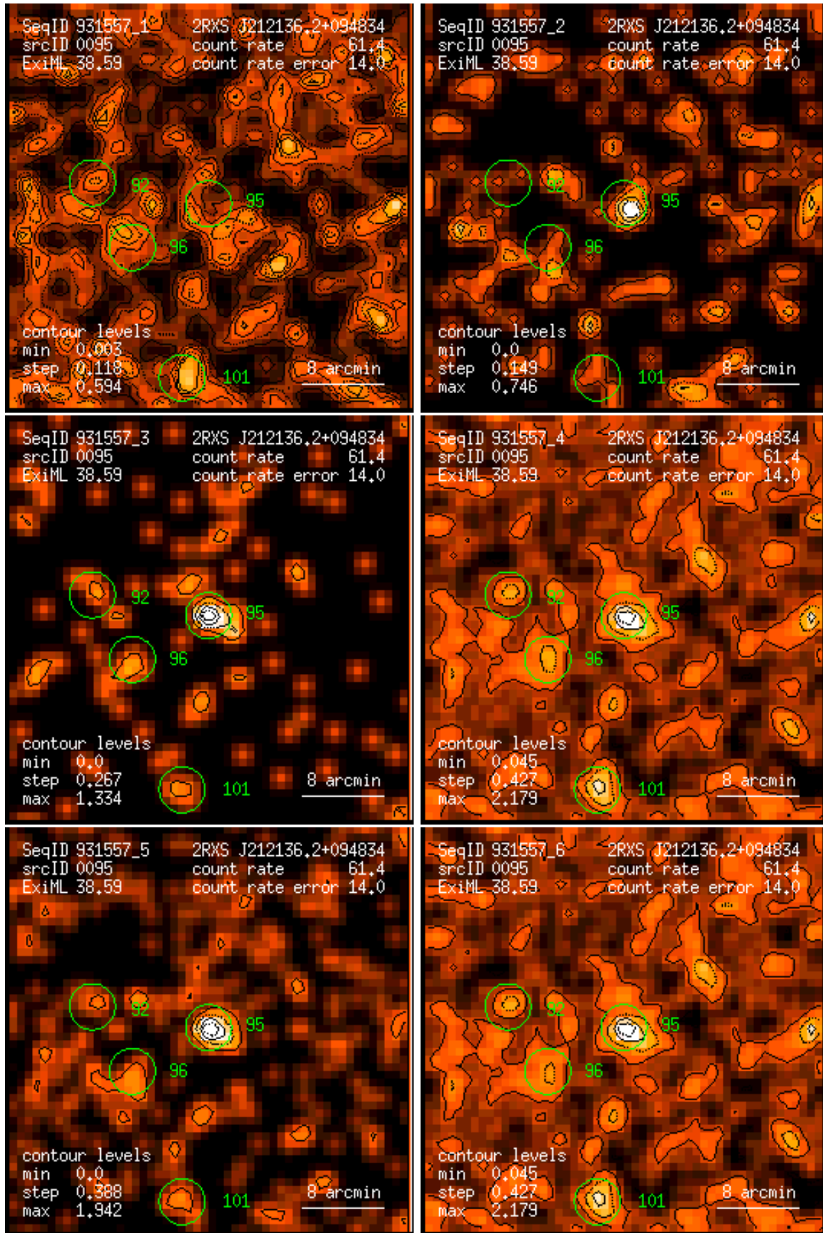
Figure 95: RASS 931557: detection 0095: band rate images, Gaussian filter: (1) PSPC channels 11 – 41, (2) 52 – 90, (3) 91 – 201, (4) 11 – 235, (5) 52 – 201, (6) 11 – 201. Broad band rates in counts/ks. Band rate contour levels in counts/ks/arcmin 2 .
