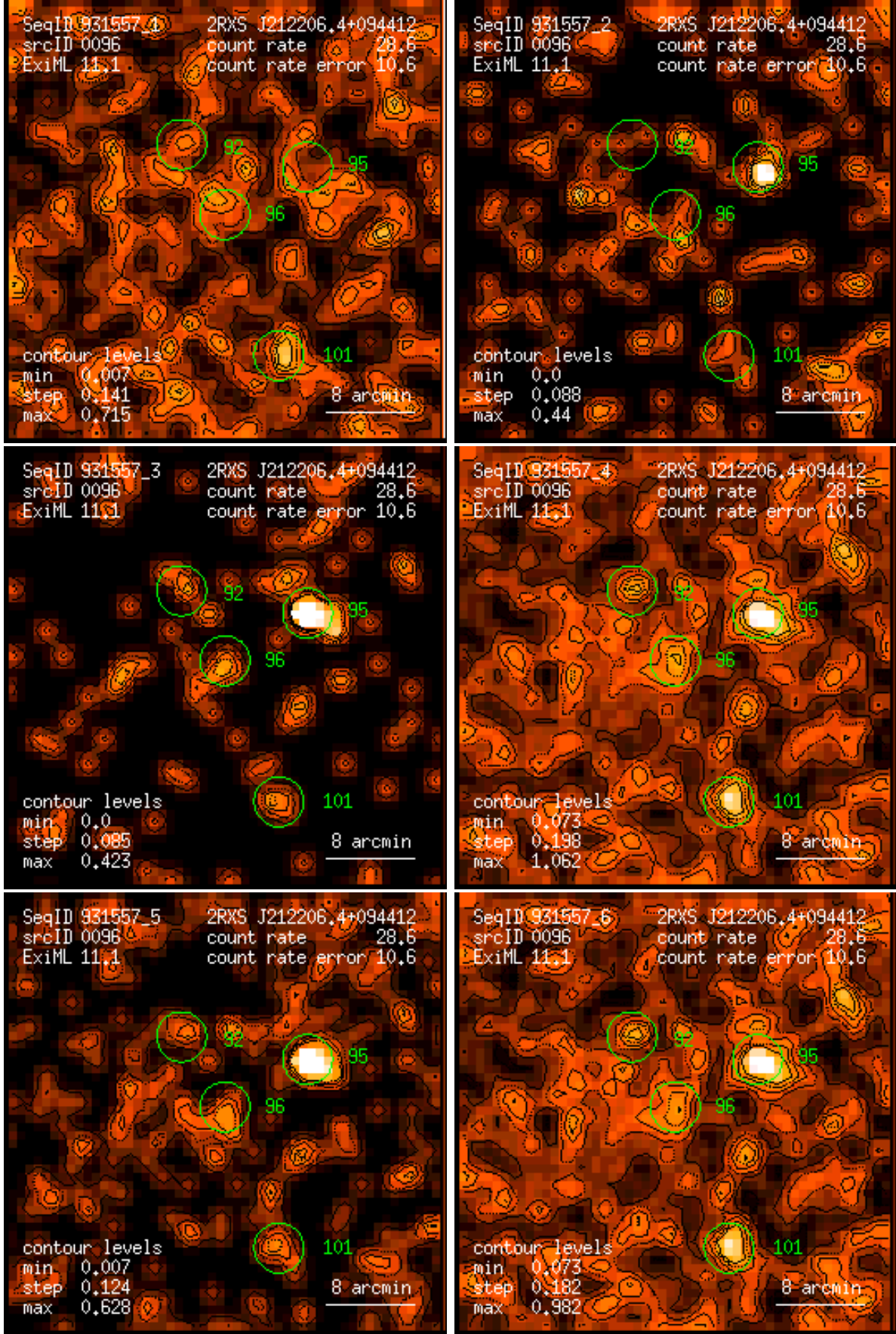
Figure 96: RASS 931557: detection 0096: band rate images, Gaussian filter: (1) PSPC channels 11 – 41, (2) 52 – 90, (3) 91 – 201, (4) 11 – 235, (5) 52 – 201, (6) 11 – 201. Broad band rates in counts/ks. Band rate contour levels in counts/ks/arcmin 2 .
