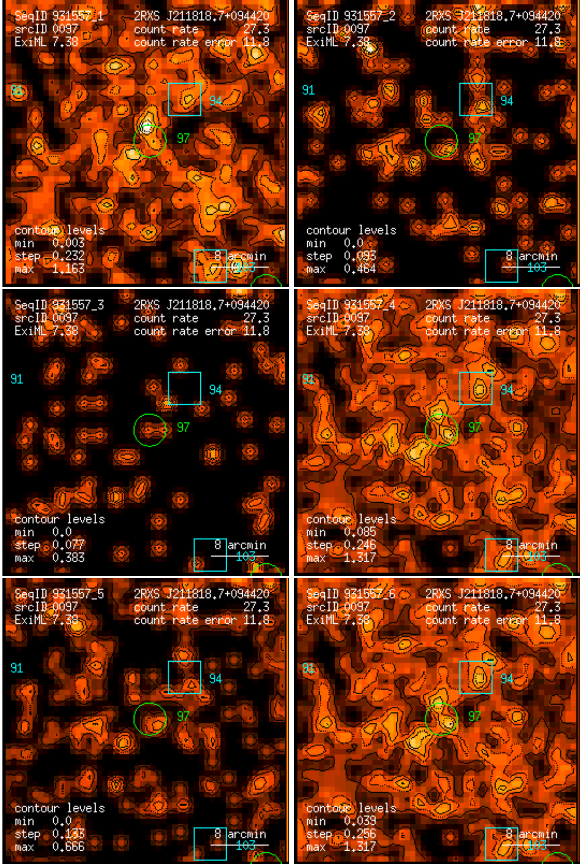
Figure 97: RASS 931557: detection 0097: band rate images, Gaussian filter: (1) PSPC channels 11 – 41, (2) 52 – 90, (3) 91 – 201, (4) 11 – 235, (5) 52 – 201, (6) 11 – 201. Broad band rates in counts/ks. Band rate contour levels in counts/ks/arcmin 2 .
