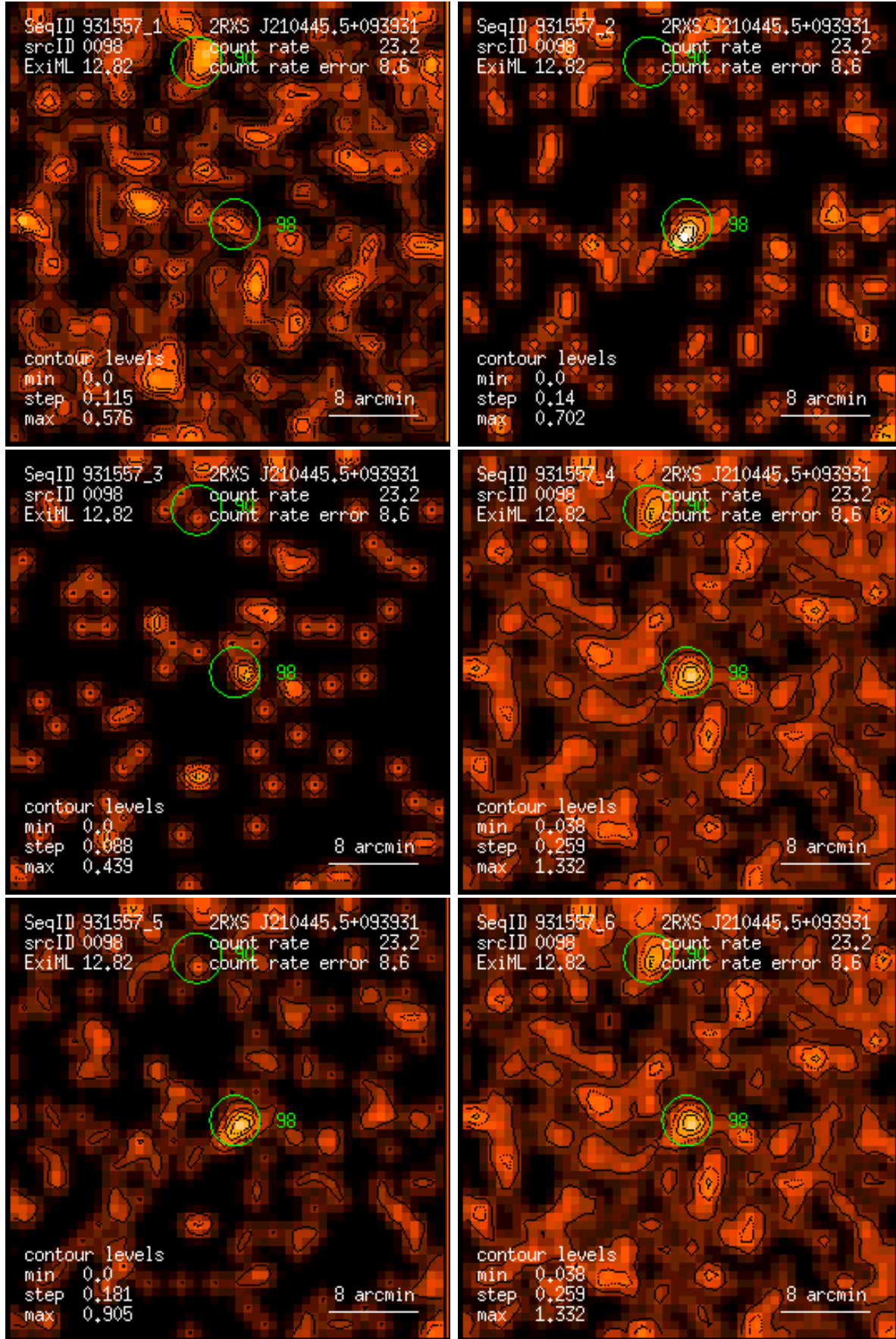
Figure 98: RASS 931557: detection 0098: band rate images, Gaussian filter: (1) PSPC channels 11 – 41, (2) 52 – 90, (3) 91 – 201, (4) 11 – 235, (5) 52 – 201, (6) 11 – 201. Broad band rates in counts/ks. Band rate contour levels in counts/ks/arcmin 2 .
