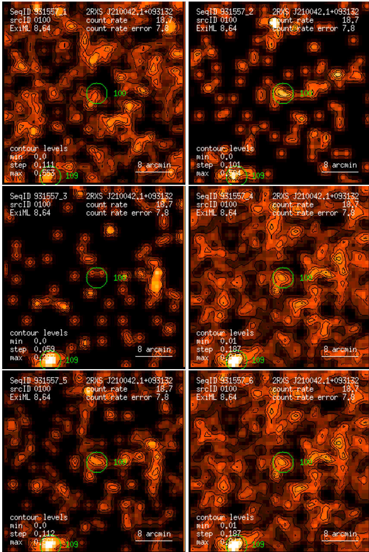
Figure 100: RASS 931557: detection 0100: band rate images, Gaussian filter: (1) PSPC channels 11 – 41, (2) 52 – 90, (3) 91 – 201, (4) 11 – 235, (5) 52 – 201, (6) 11 – 201. Broad band rates in counts/ks. Band rate contour levels in counts/ks/arcmin 2 .
