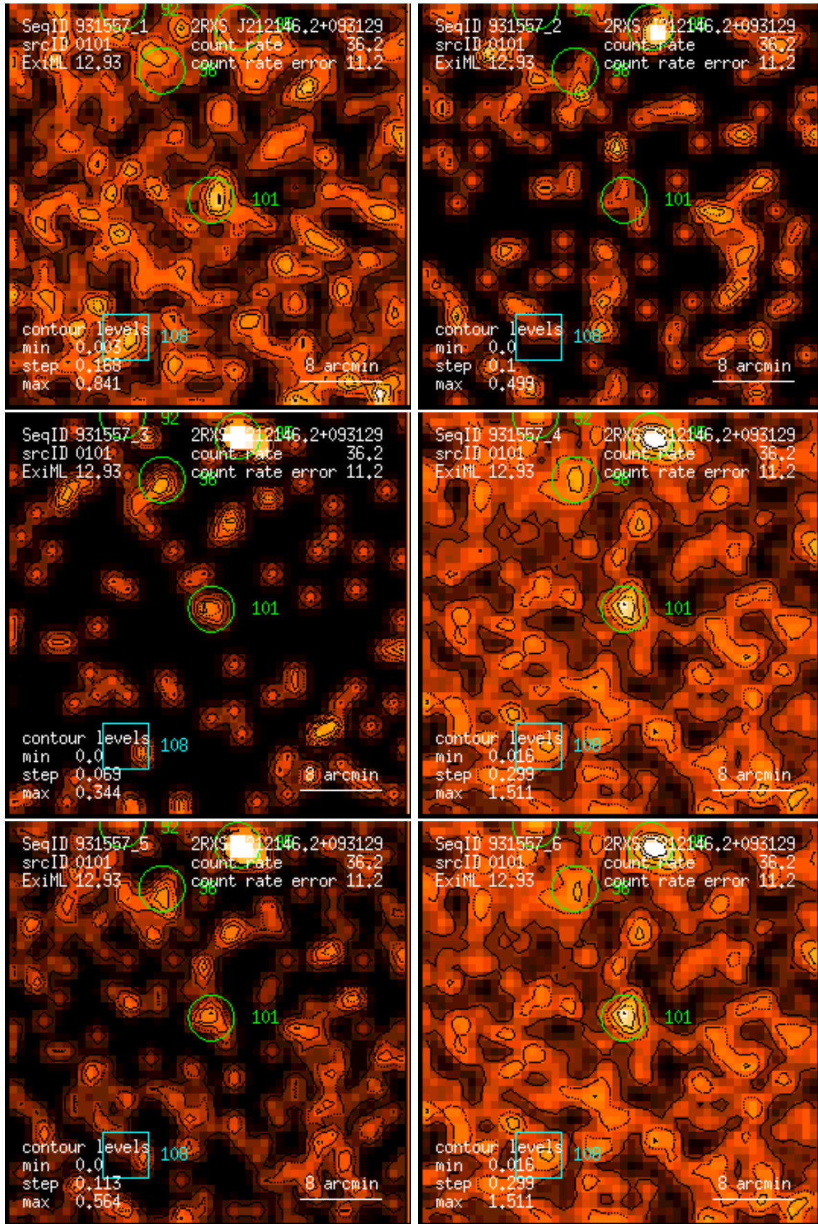
Figure 101: RASS 931557: detection 0101: band rate images, Gaussian filter: (1) PSPC channels 11 – 41, (2) 52 – 90, (3) 91 – 201, (4) 11 – 235, (5) 52 – 201, (6) 11 – 201. Broad band rates in counts/ks. Band rate contour levels in counts/ks/arcmin 2 .
