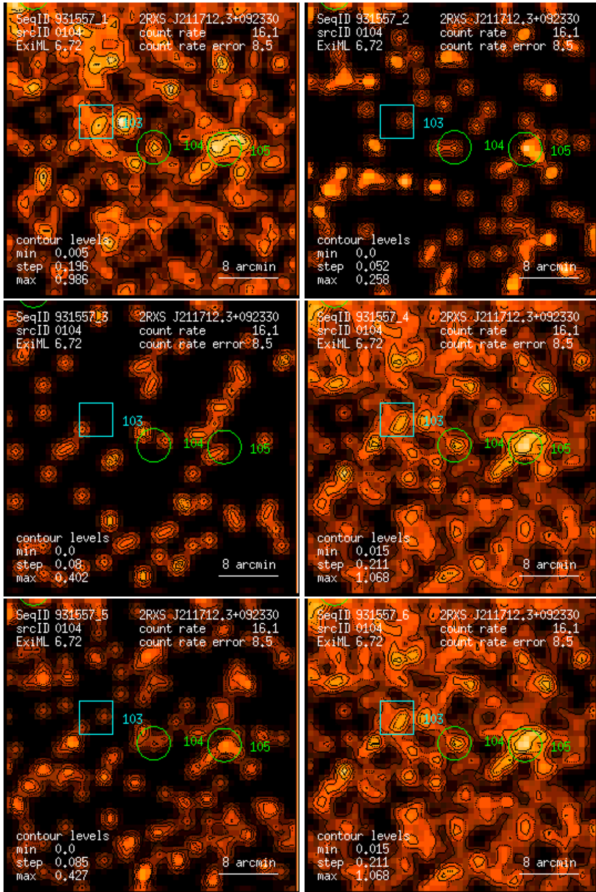
Figure 104: RASS 931557: detection 0104: band rate images, Gaussian filter: (1) PSPC channels 11 – 41, (2) 52 – 90, (3) 91 – 201, (4) 11 – 235, (5) 52 – 201, (6) 11 – 201. Broad band rates in counts/ks. Band rate contour levels in counts/ks/arcmin 2 .
