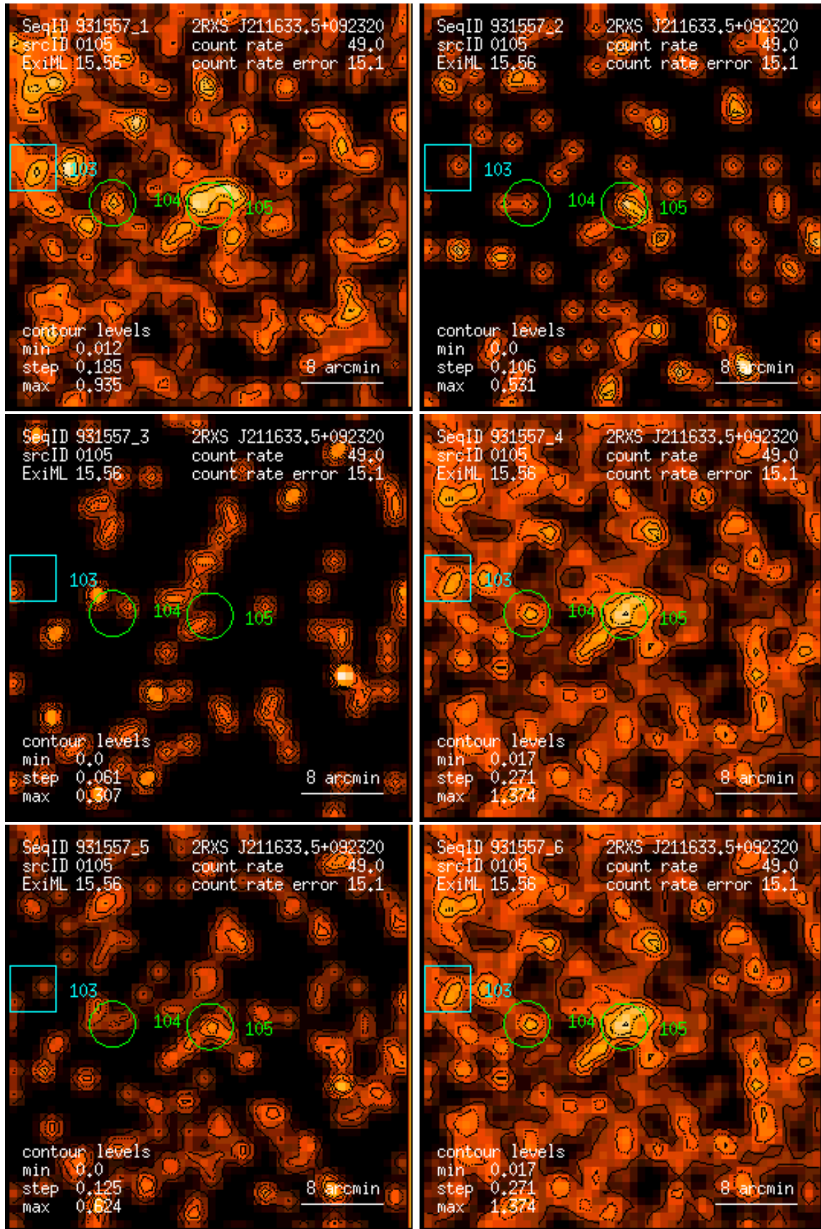
Figure 105: RASS 931557: detection 0105: band rate images, Gaussian filter: (1) PSPC channels 11 – 41, (2) 52 – 90, (3) 91 – 201, (4) 11 – 235, (5) 52 – 201, (6) 11 – 201. Broad band rates in counts/ks. Band rate contour levels in counts/ks/arcmin 2 .
