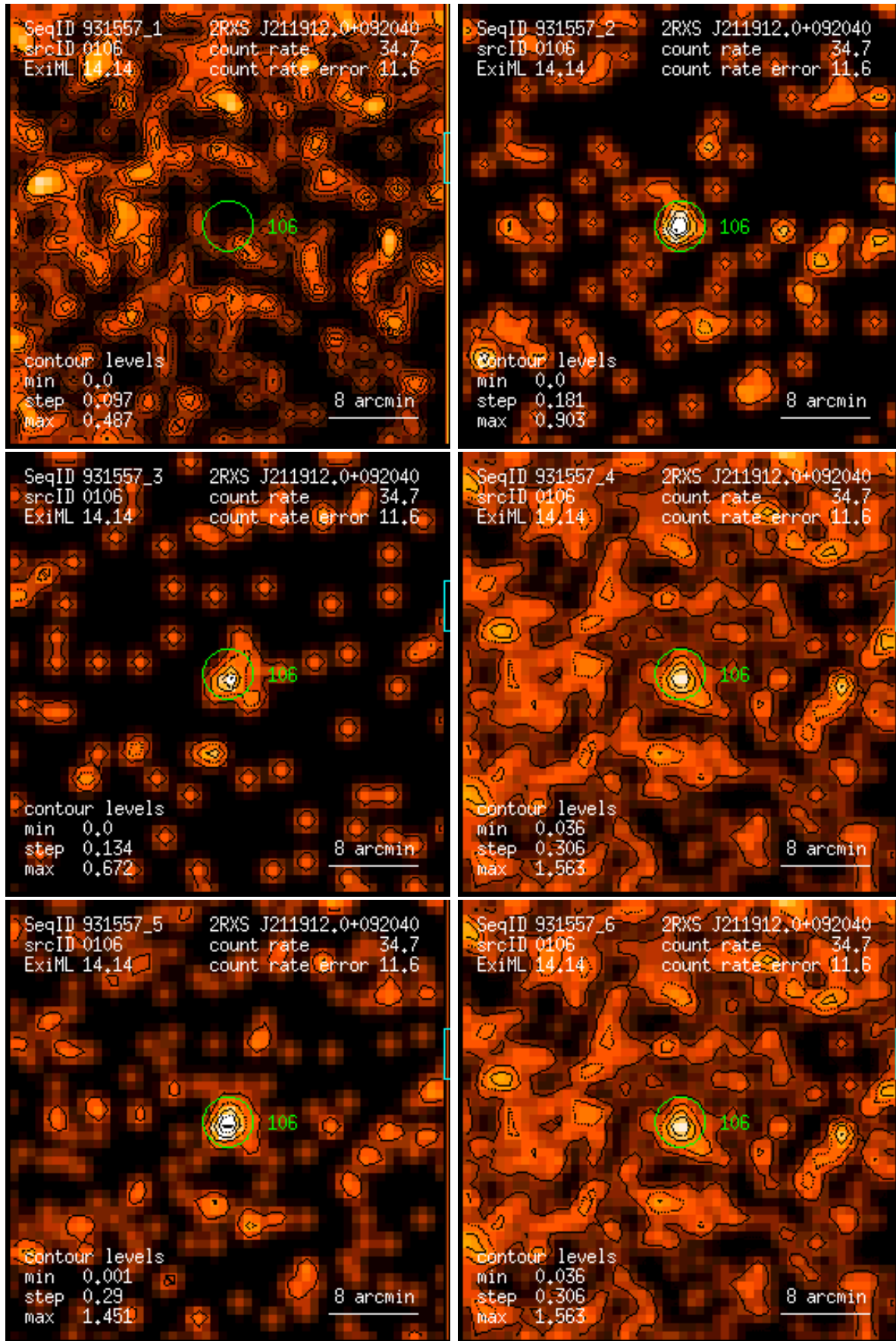
Figure 106: RASS 931557: detection 0106: band rate images, Gaussian filter: (1) PSPC channels 11 – 41, (2) 52 – 90, (3) 91 – 201, (4) 11 – 235, (5) 52 – 201, (6) 11 – 201. Broad band rates in counts/ks. Band rate contour levels in counts/ks/arcmin 2 .
