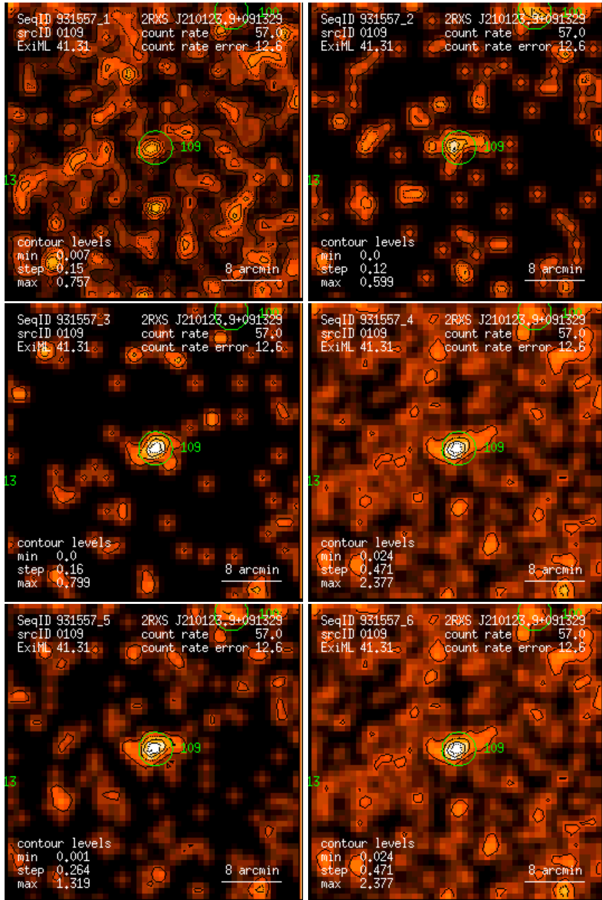
Figure 109: RASS 931557: detection 0109: band rate images, Gaussian filter: (1) PSPC channels 11 – 41, (2) 52 – 90, (3) 91 – 201, (4) 11 – 235, (5) 52 – 201, (6) 11 – 201. Broad band rates in counts/ks. Band rate contour levels in counts/ks/arcmin 2 .
