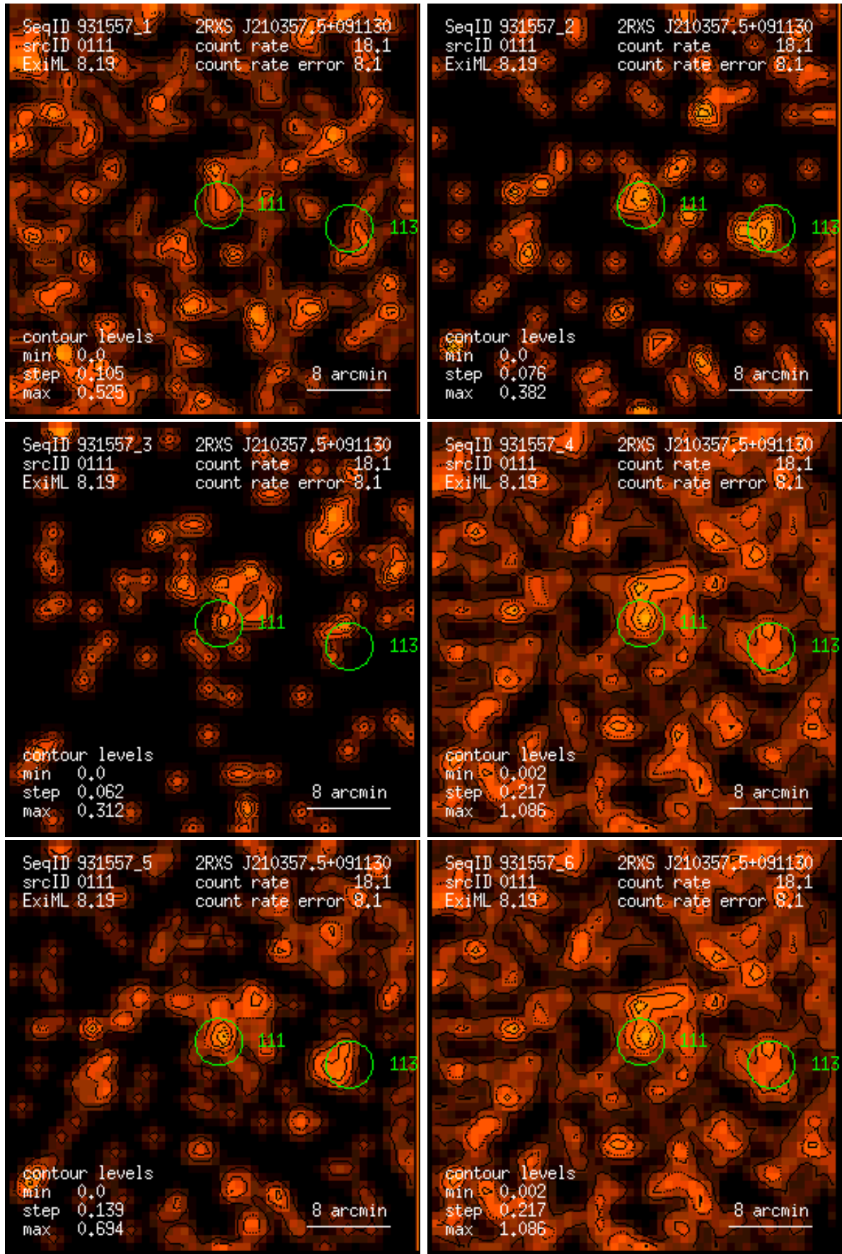
Figure 111: RASS 931557: detection 0111: band rate images, Gaussian filter: (1) PSPC channels 11 – 41, (2) 52 – 90, (3) 91 – 201, (4) 11 – 235, (5) 52 – 201, (6) 11 – 201. Broad band rates in counts/ks. Band rate contour levels in counts/ks/arcmin 2 .
