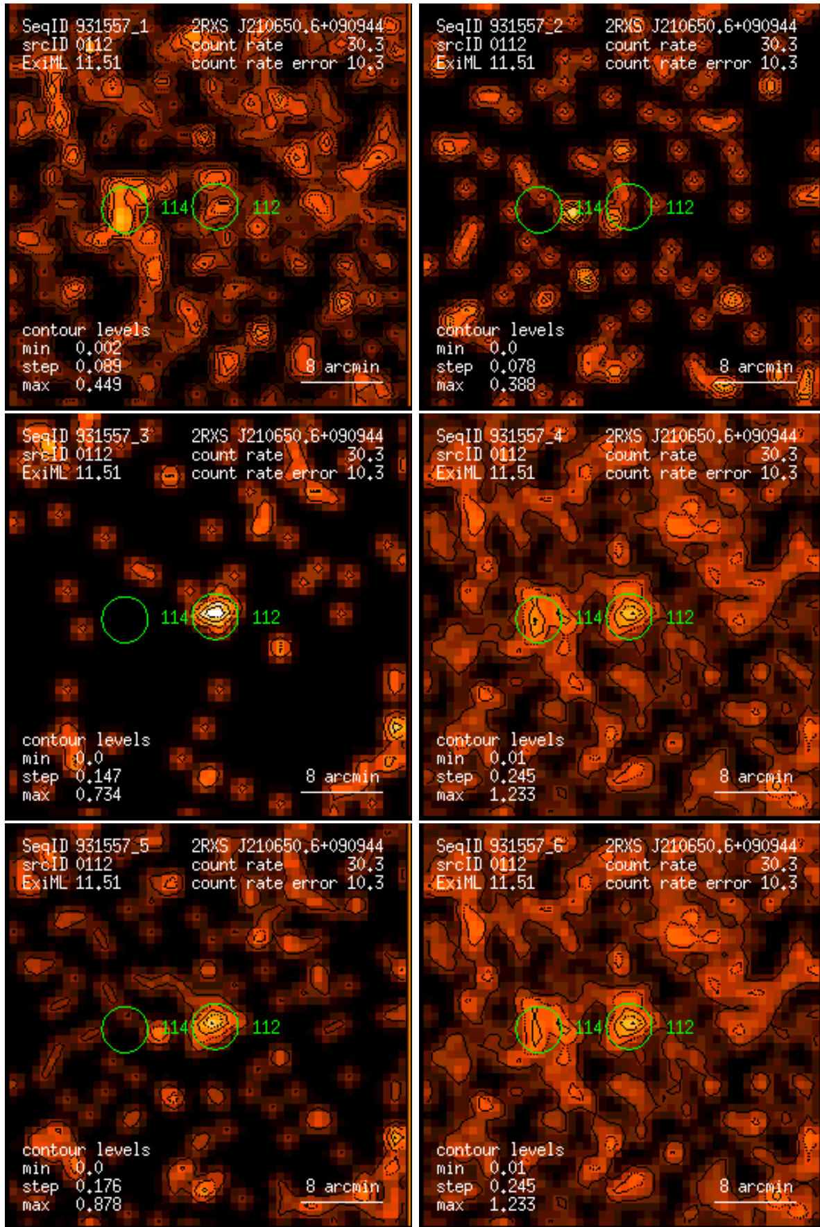
Figure 112: RASS 931557: detection 0112: band rate images, Gaussian filter: (1) PSPC channels 11 – 41, (2) 52 – 90, (3) 91 – 201, (4) 11 – 235, (5) 52 – 201, (6) 11 – 201. Broad band rates in counts/ks. Band rate contour levels in counts/ks/arcmin 2 .
