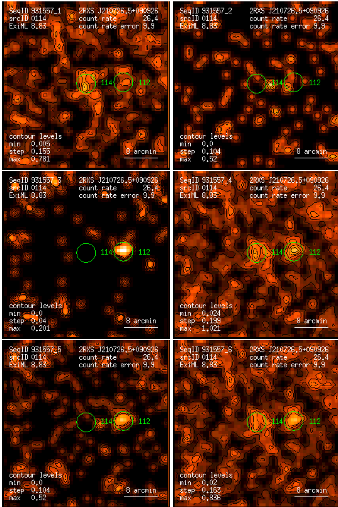
Figure 114: RASS 931557: detection 0114: band rate images, Gaussian filter: (1) PSPC channels 11 – 41, (2) 52 – 90, (3) 91 – 201, (4) 11 – 235, (5) 52 – 201, (6) 11 – 201. Broad band rates in counts/ks. Band rate contour levels in counts/ks/arcmin 2 .
