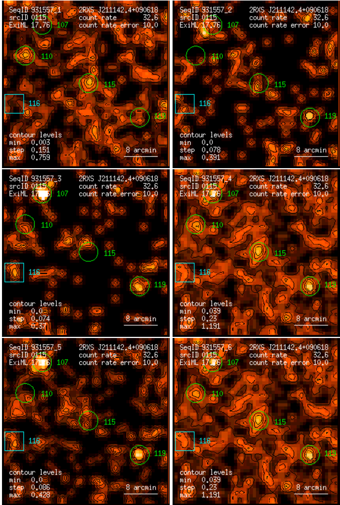
Figure 115: RASS 931557: detection 0115: band rate images, Gaussian filter: (1) PSPC channels 11 – 41, (2) 52 – 90, (3) 91 – 201, (4) 11 – 235, (5) 52 – 201, (6) 11 – 201. Broad band rates in counts/ks. Band rate contour levels in counts/ks/arcmin 2 .
