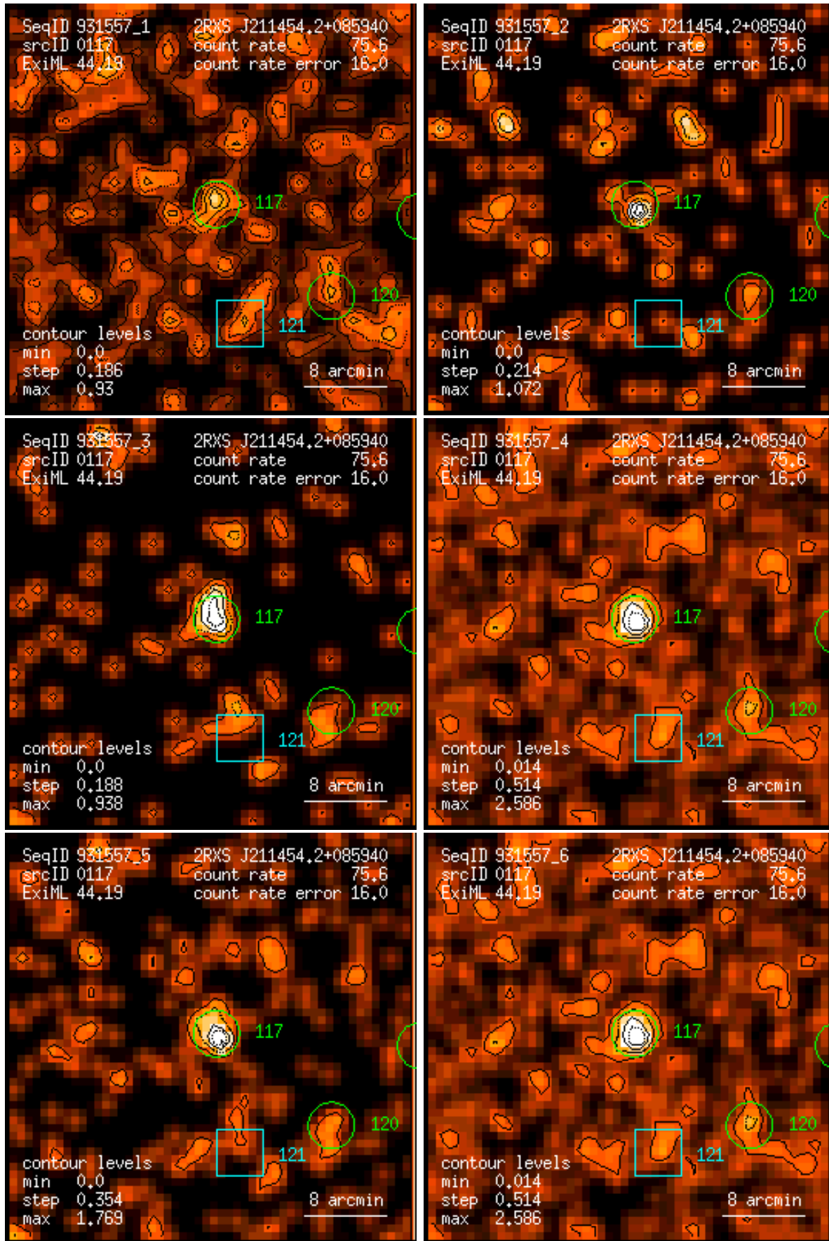
Figure 117: RASS 931557: detection 0117: band rate images, Gaussian filter: (1) PSPC channels 11 – 41, (2) 52 – 90, (3) 91 – 201, (4) 11 – 235, (5) 52 – 201, (6) 11 – 201. Broad band rates in counts/ks. Band rate contour levels in counts/ks/arcmin 2 .
