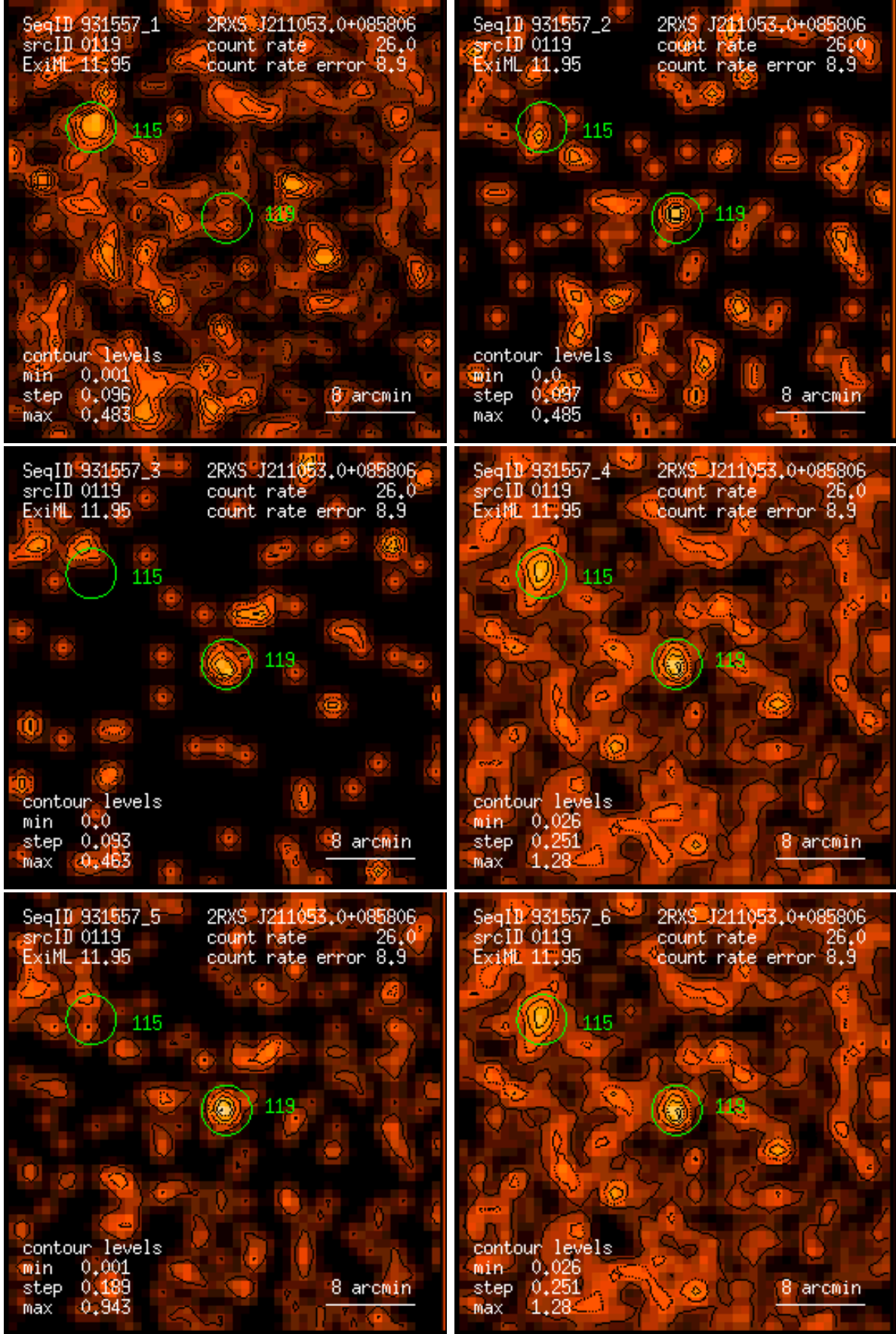
Figure 119: RASS 931557: detection 0119: band rate images, Gaussian filter: (1) PSPC channels 11 – 41, (2) 52 – 90, (3) 91 – 201, (4) 11 – 235, (5) 52 – 201, (6) 11 – 201. Broad band rates in counts/ks. Band rate contour levels in counts/ks/arcmin 2 .
