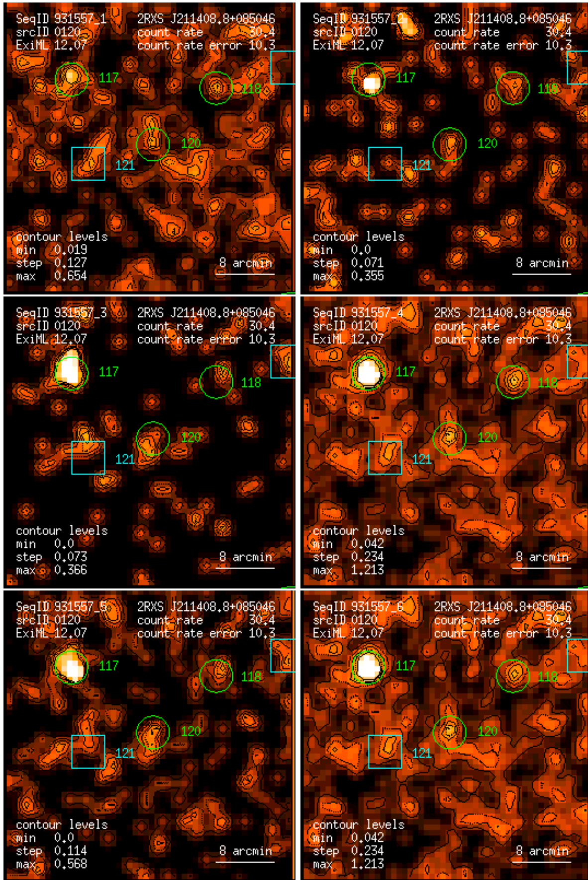
Figure 120: RASS 931557: detection 0120: band rate images, Gaussian filter: (1) PSPC channels 11 – 41, (2) 52 – 90, (3) 91 – 201, (4) 11 – 235, (5) 52 – 201, (6) 11 – 201. Broad band rates in counts/ks. Band rate contour levels in counts/ks/arcmin 2 .
