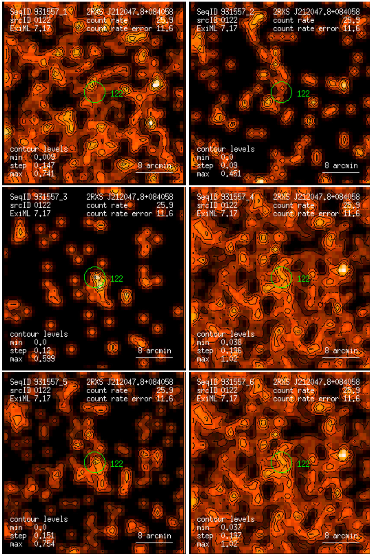
Figure 122: RASS 931557: detection 0122: band rate images, Gaussian filter: (1) PSPC channels 11 – 41, (2) 52 – 90, (3) 91 – 201, (4) 11 – 235, (5) 52 – 201, (6) 11 – 201. Broad band rates in counts/ks. Band rate contour levels in counts/ks/arcmin 2 .
