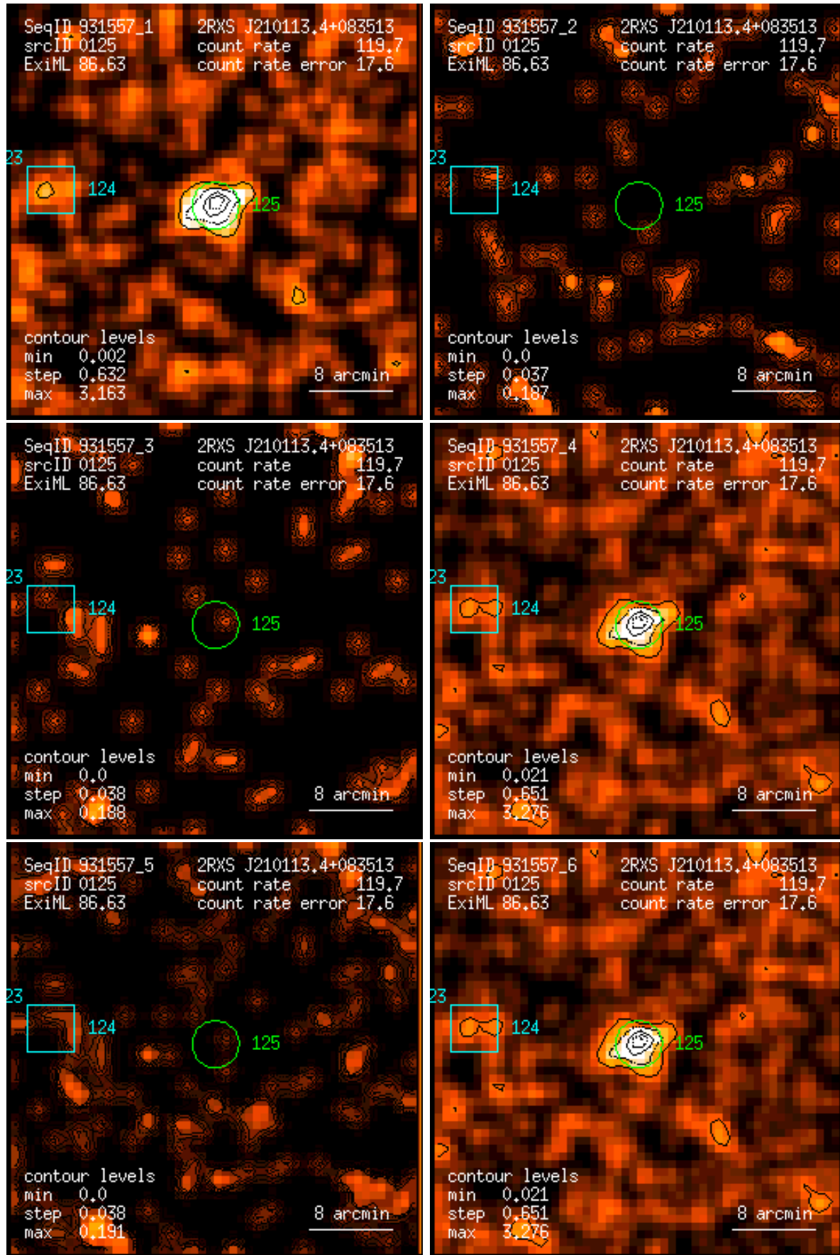
Figure 125: RASS 931557: detection 0125: band rate images, Gaussian filter: (1) PSPC channels 11 – 41, (2) 52 – 90, (3) 91 – 201, (4) 11 – 235, (5) 52 – 201, (6) 11 – 201. Broad band rates in counts/ks. Band rate contour levels in counts/ks/arcmin 2 .
