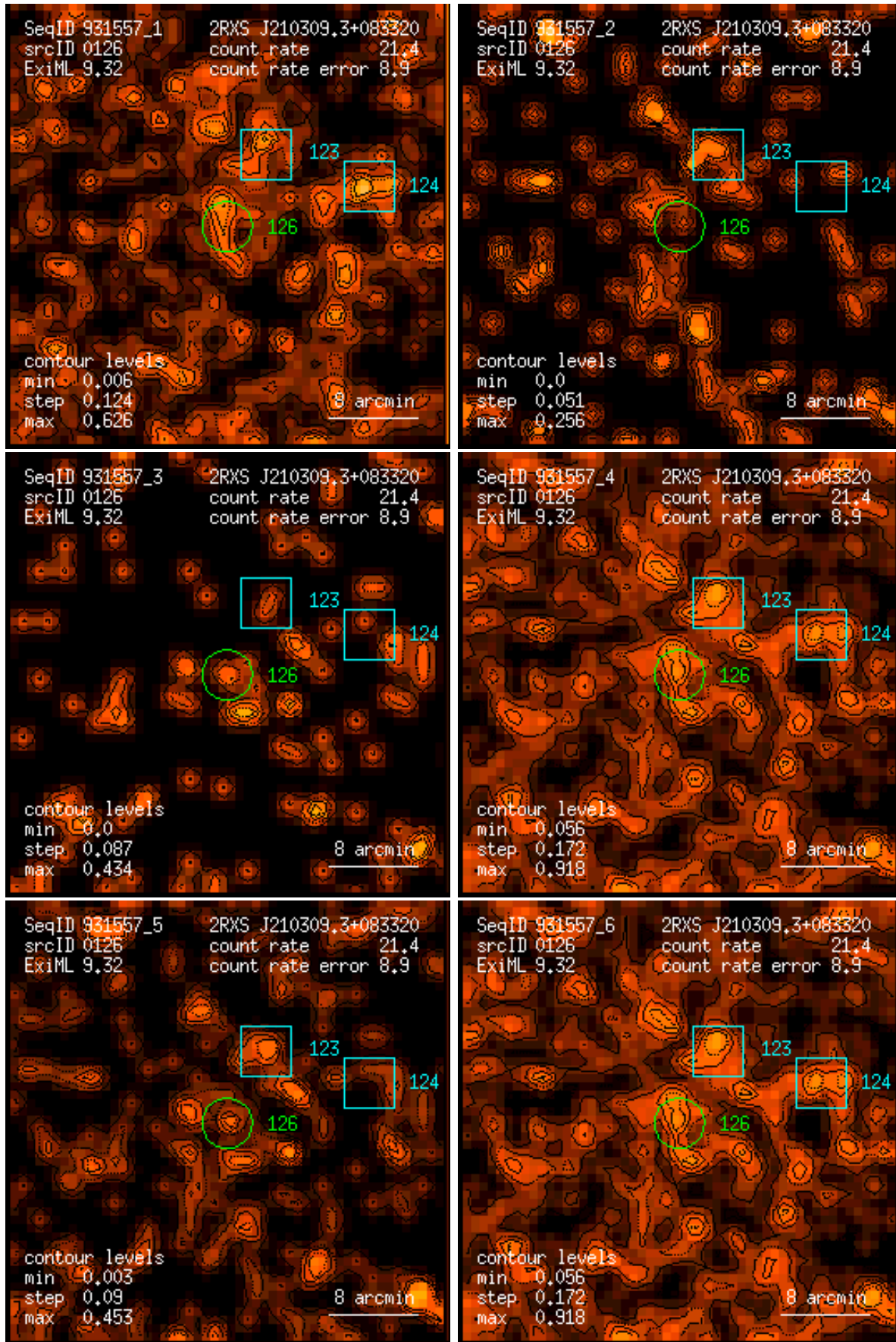
Figure 126: RASS 931557: detection 0126: band rate images, Gaussian filter: (1) PSPC channels 11 – 41, (2) 52 – 90, (3) 91 – 201, (4) 11 – 235, (5) 52 – 201, (6) 11 – 201. Broad band rates in counts/ks. Band rate contour levels in counts/ks/arcmin 2 .
