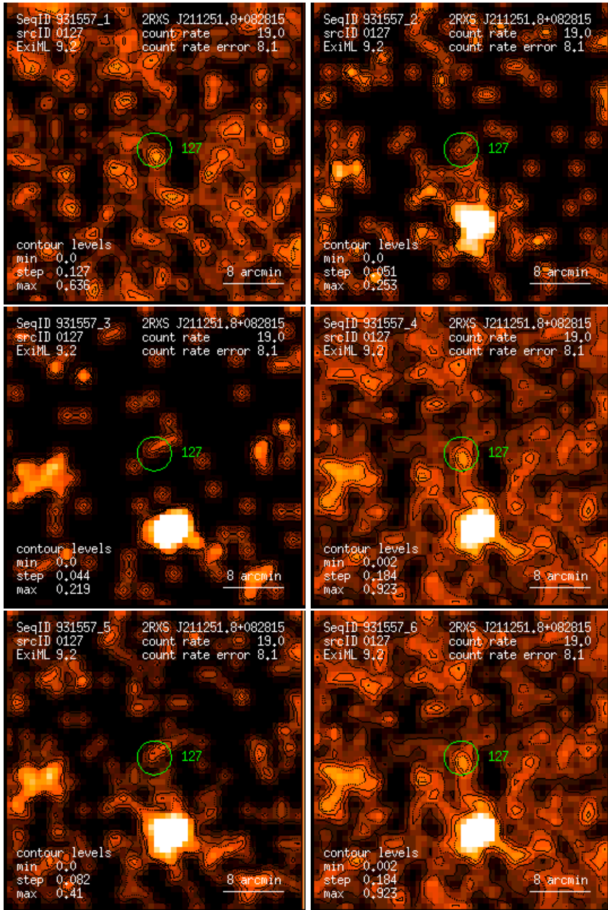
Figure 127: RASS 931557: detection 0127: band rate images, Gaussian filter: (1) PSPC channels 11 – 41, (2) 52 – 90, (3) 91 – 201, (4) 11 – 235, (5) 52 – 201, (6) 11 – 201. Broad band rates in counts/ks. Band rate contour levels in counts/ks/arcmin 2 .
