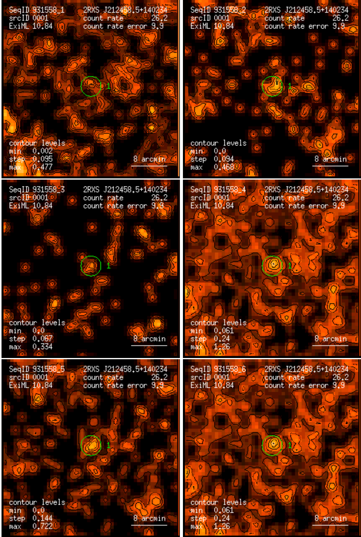
Figure 1: RASS 931558: detection 0001: band rate images, Gaussian filter: (1) PSPC channels 11 – 41, (2) 52 – 90, (3) 91 – 201, (4) 11 – 235, (5) 52 – 201, (6) 11 – 201. Broad band rates in counts/ks. Band rate contour levels in counts/ks/arcmin 2 .
