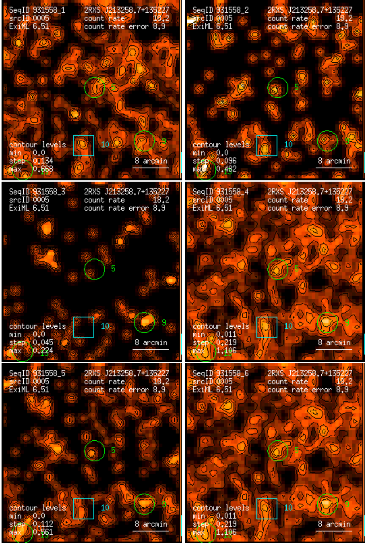
Figure 5: RASS 931558: detection 0005: band rate images, Gaussian filter: (1) PSPC channels 11 – 41, (2) 52 – 90, (3) 91 – 201, (4) 11 – 235, (5) 52 – 201, (6) 11 – 201. Broad band rates in counts/ks. Band rate contour levels in counts/ks/arcmin 2 .
